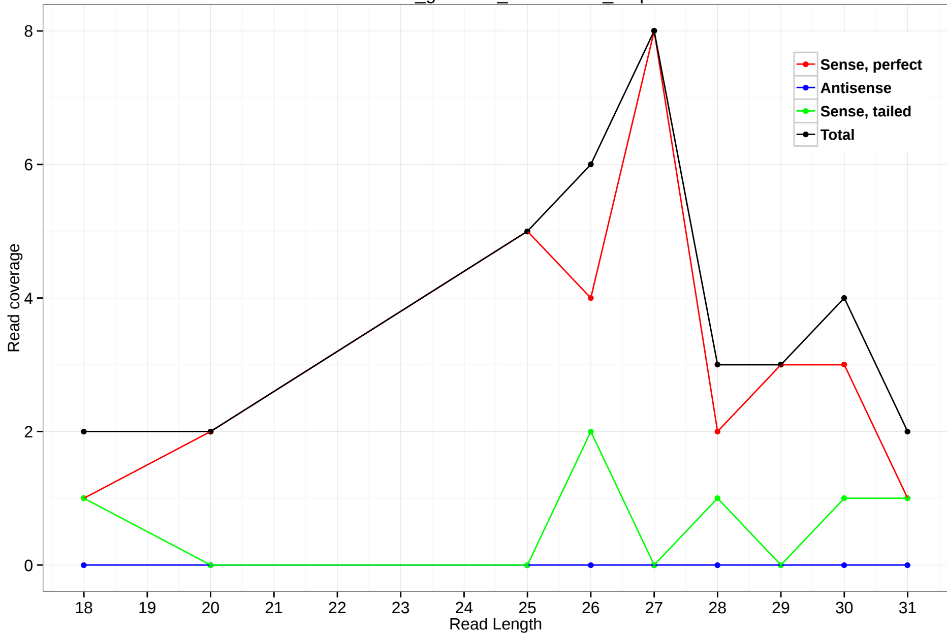
rheMac3_genscan_chr11.2206_1.3p
