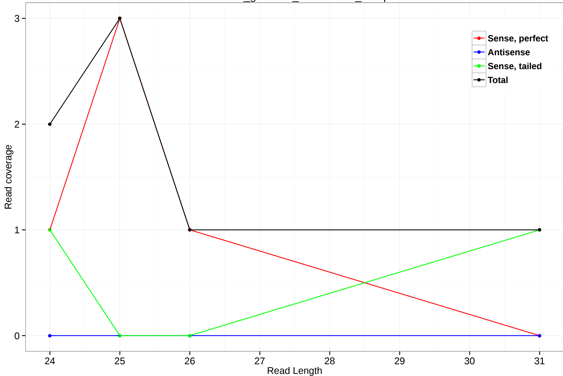
rheMac3_genscan_chr11.2204_30.3p
