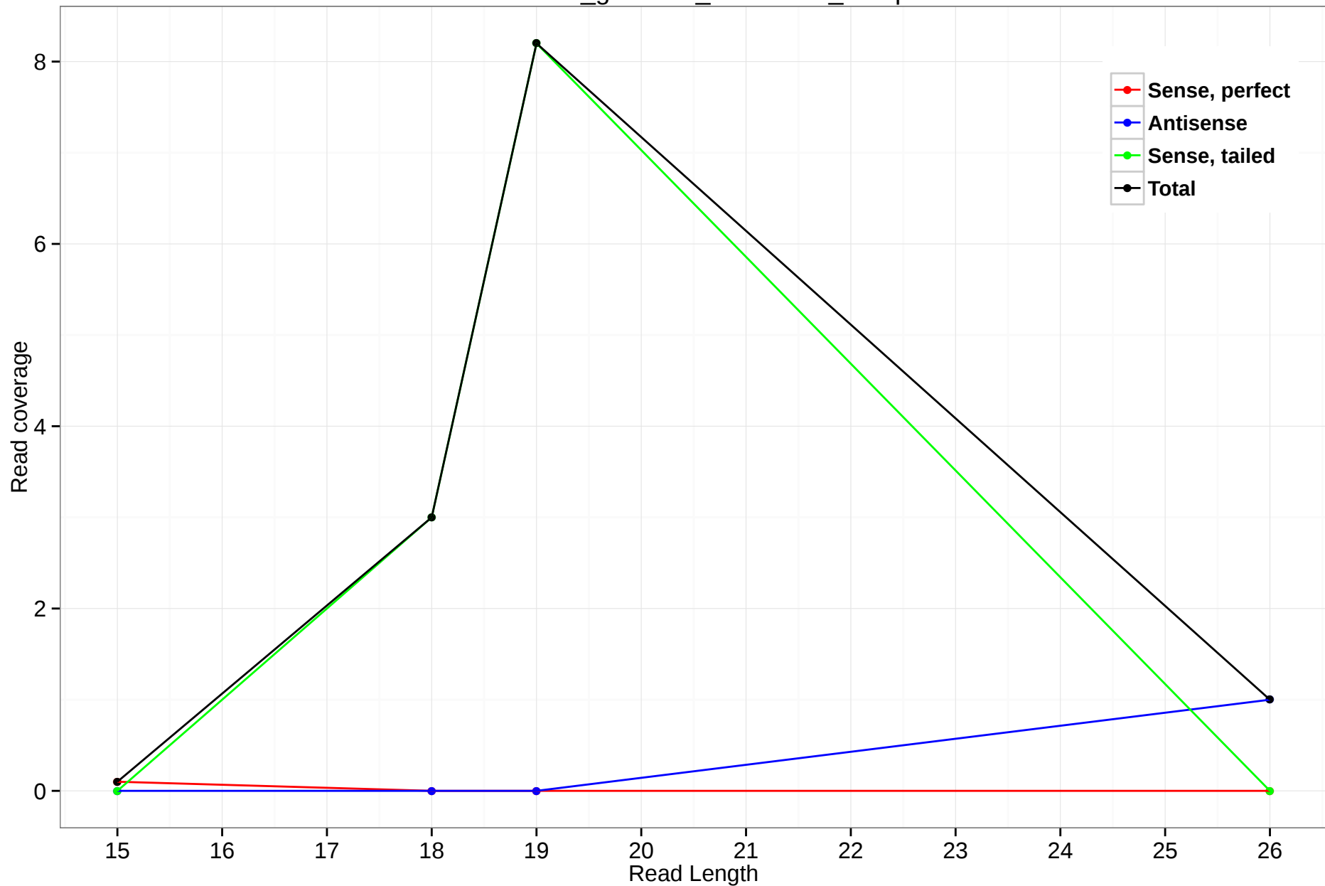
rheMac3_genscan_chr11.219_80.5p
