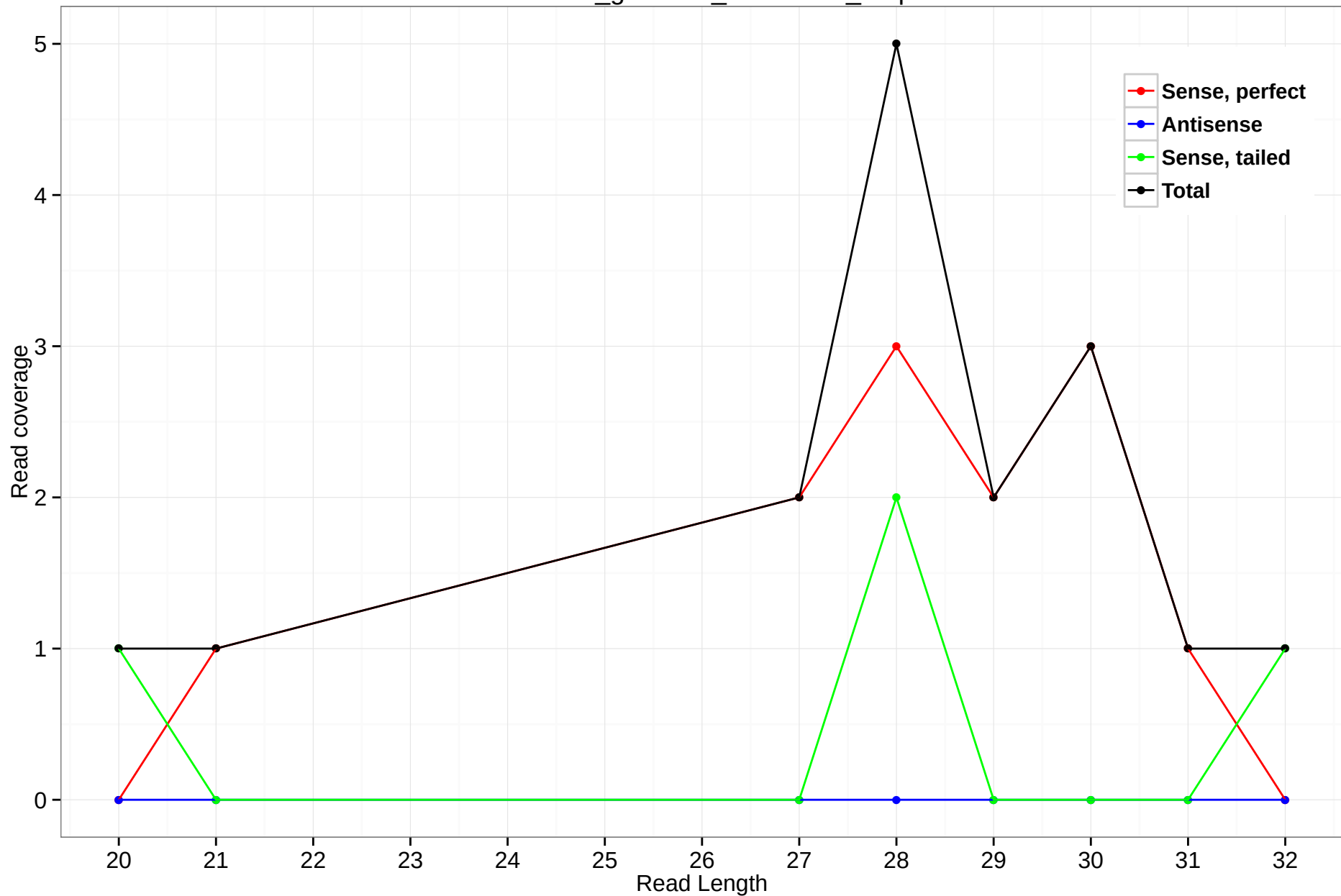
rheMac3_genscan_chr11.216_2.5p
