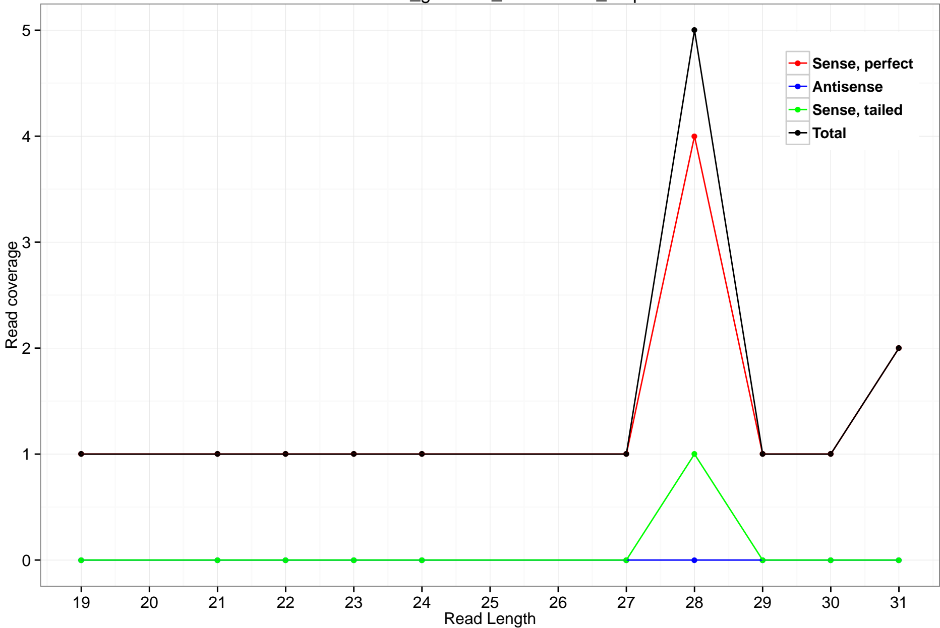
rheMac3_genscan_chr11.2160_2.5p
