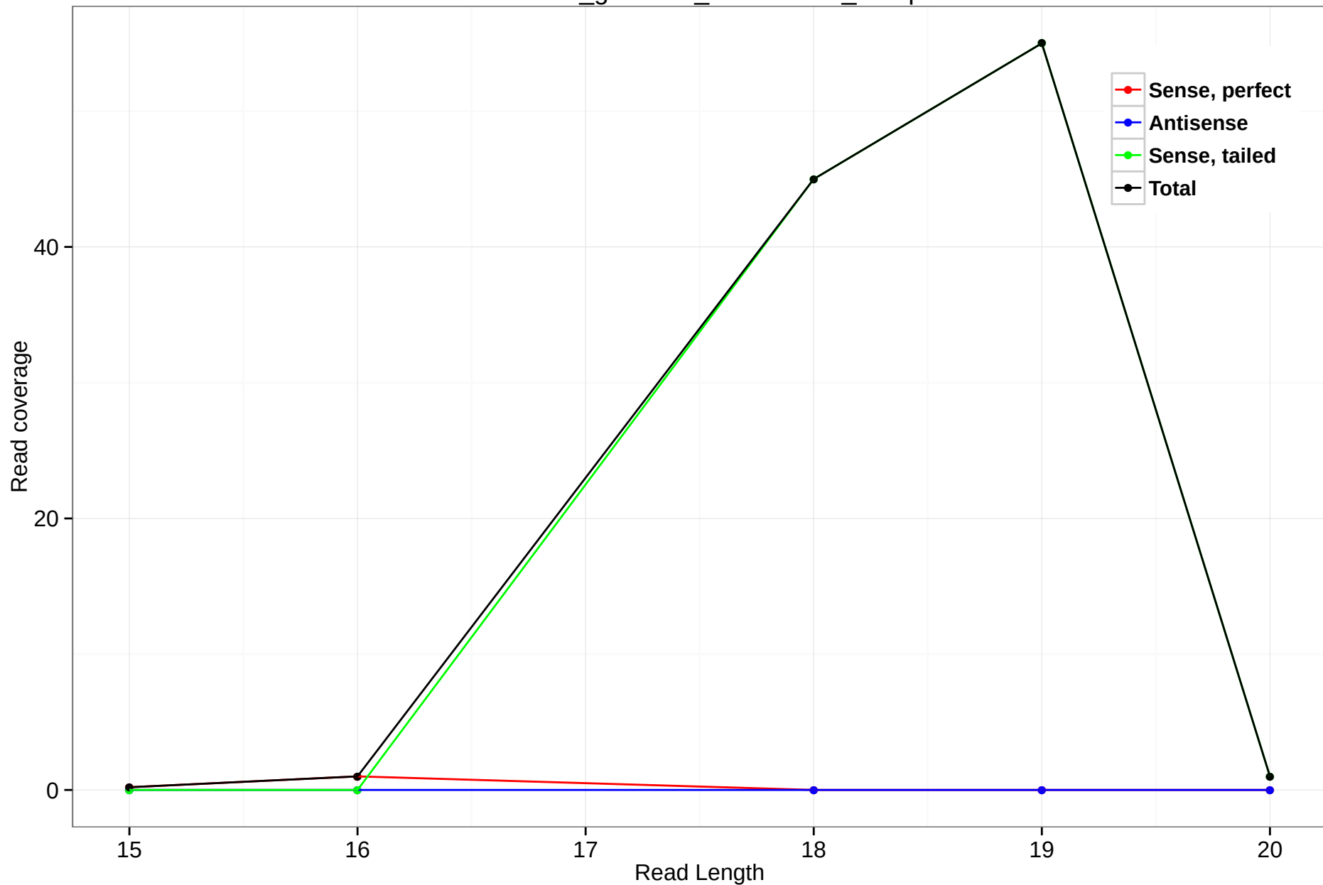
rheMac3_genscan_chr11.2156_14.3p
