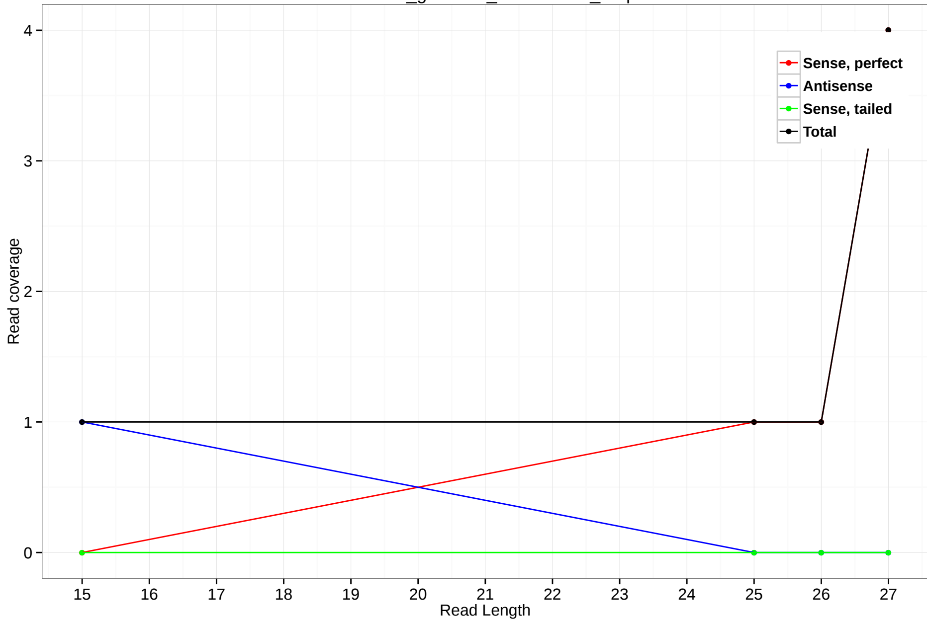
rheMac3_genscan_chr11.2135_3.5p
