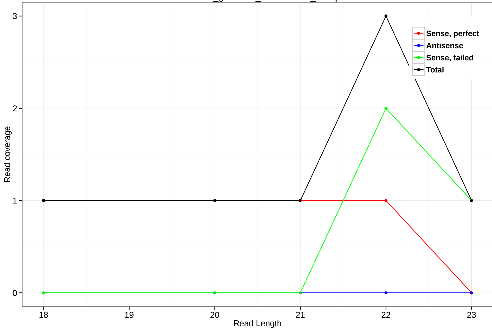
rheMac3_genscan_chr11.2135_26.3p
