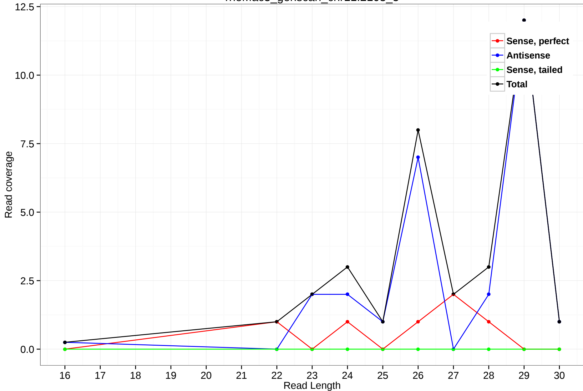
rheMac3_genscan_chr11.2103_5
