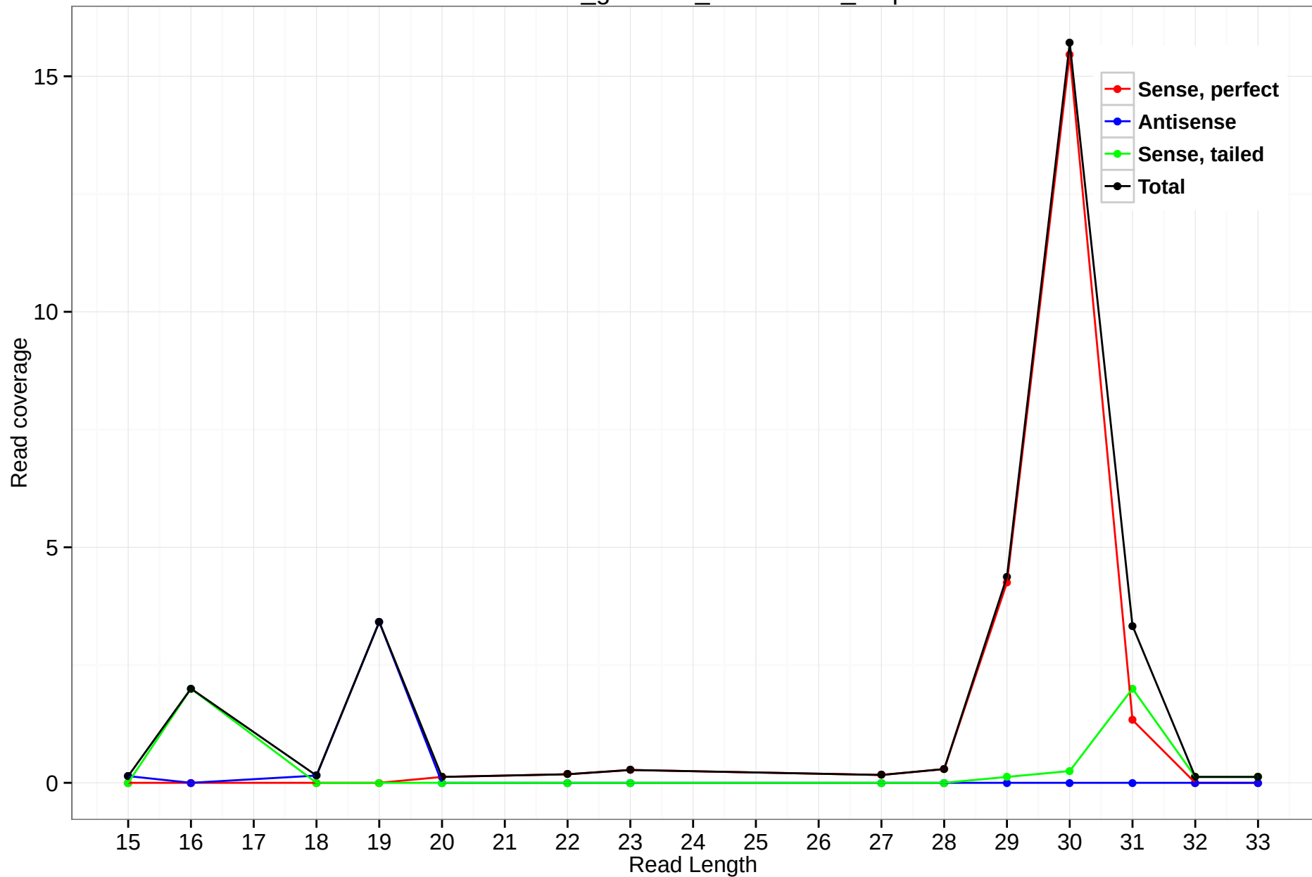
rheMac3_genscan_chr11.2096_2.5p
