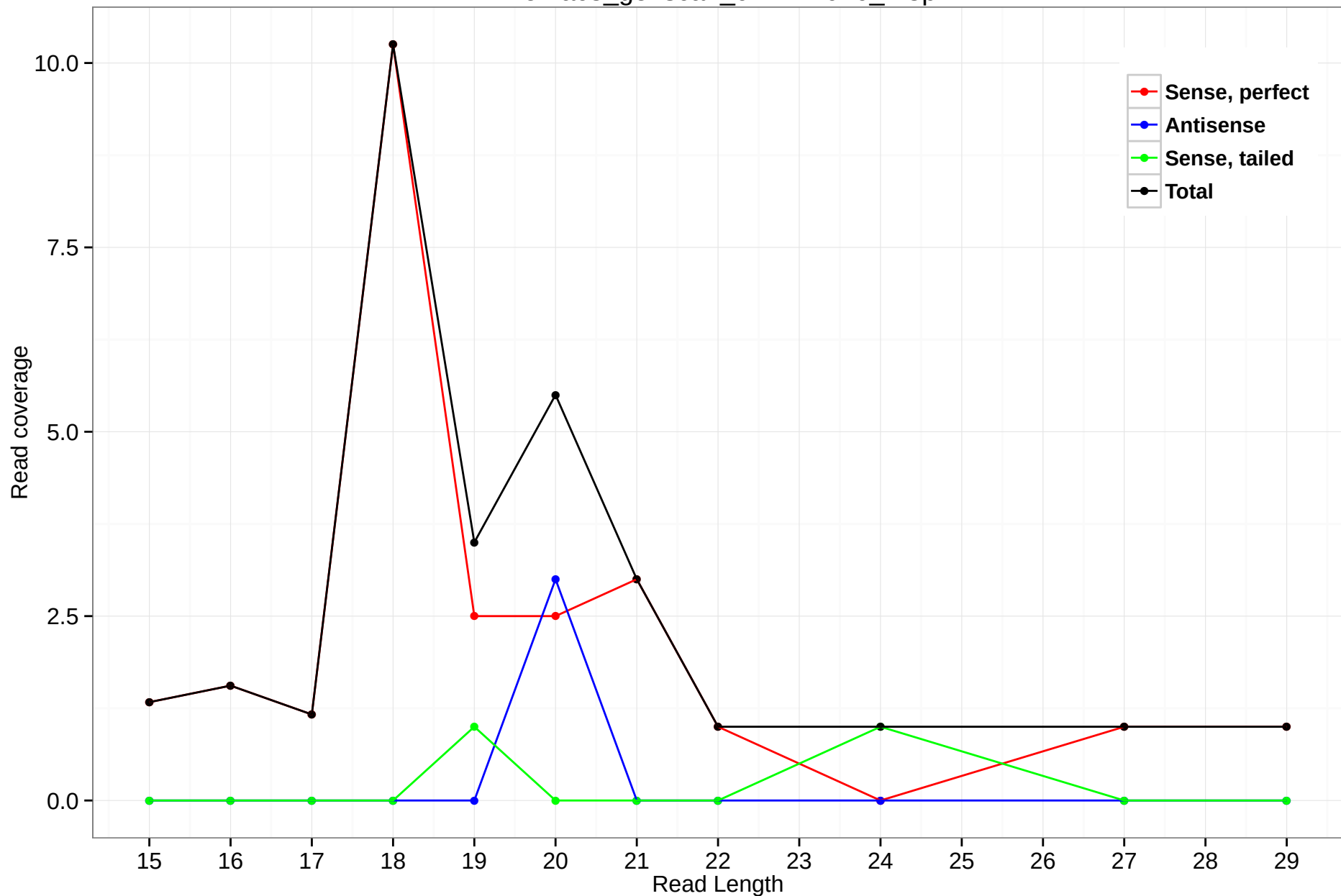
rheMac3_genscan_chr11.2076_1.3p
