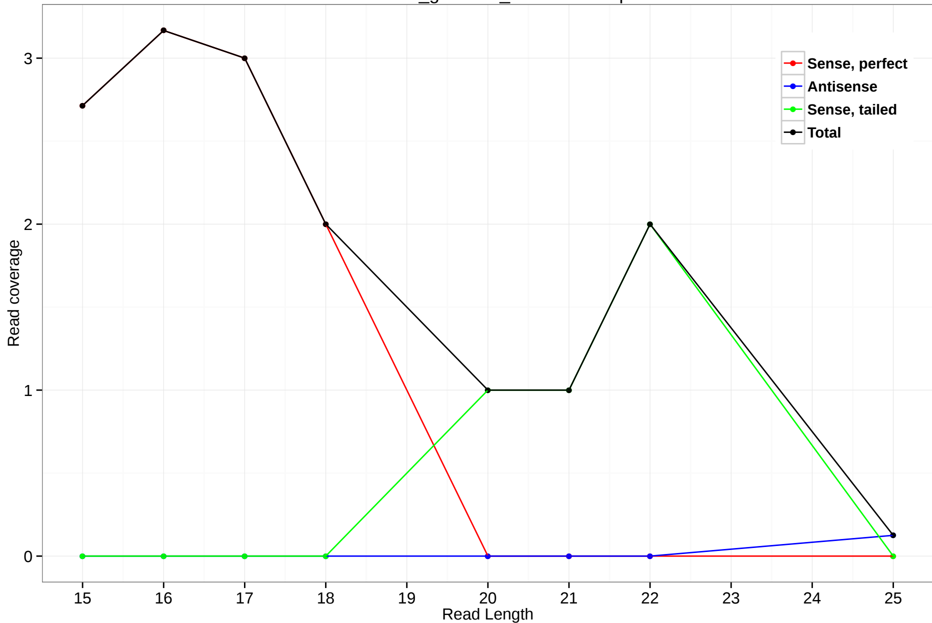
rheMac3_genscan_chr11.2061.3p
