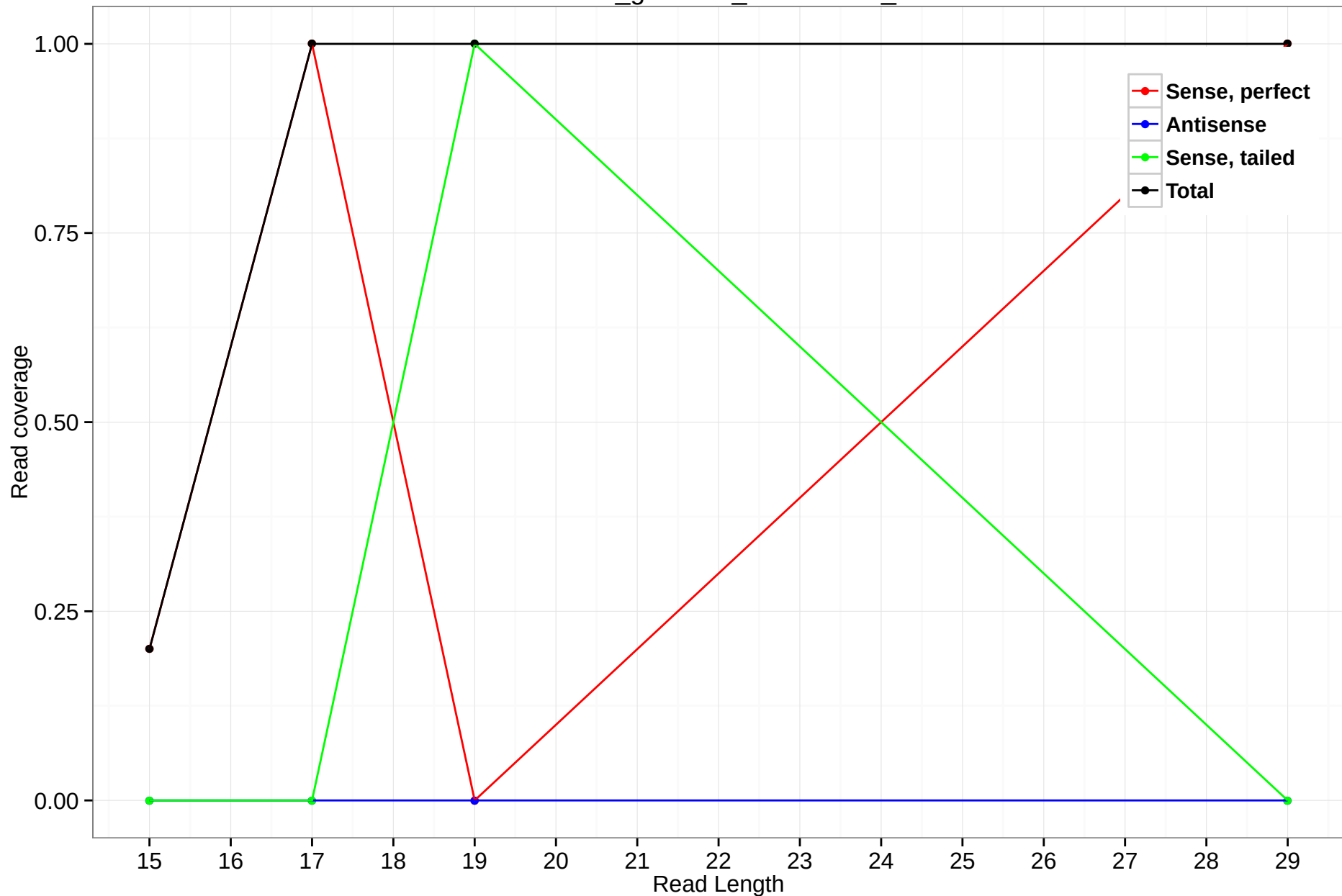
rheMac3_genscan_chr11.2060_47
