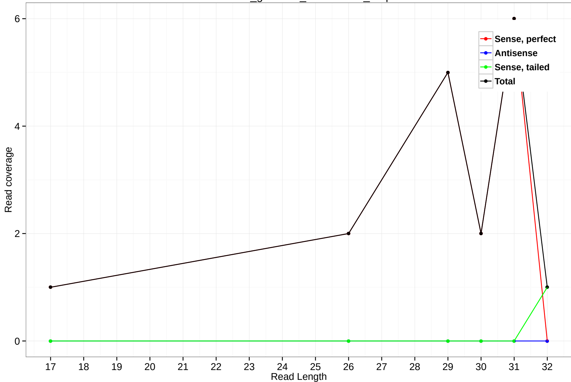
rheMac3_genscan_chr11.2038_3.5p
