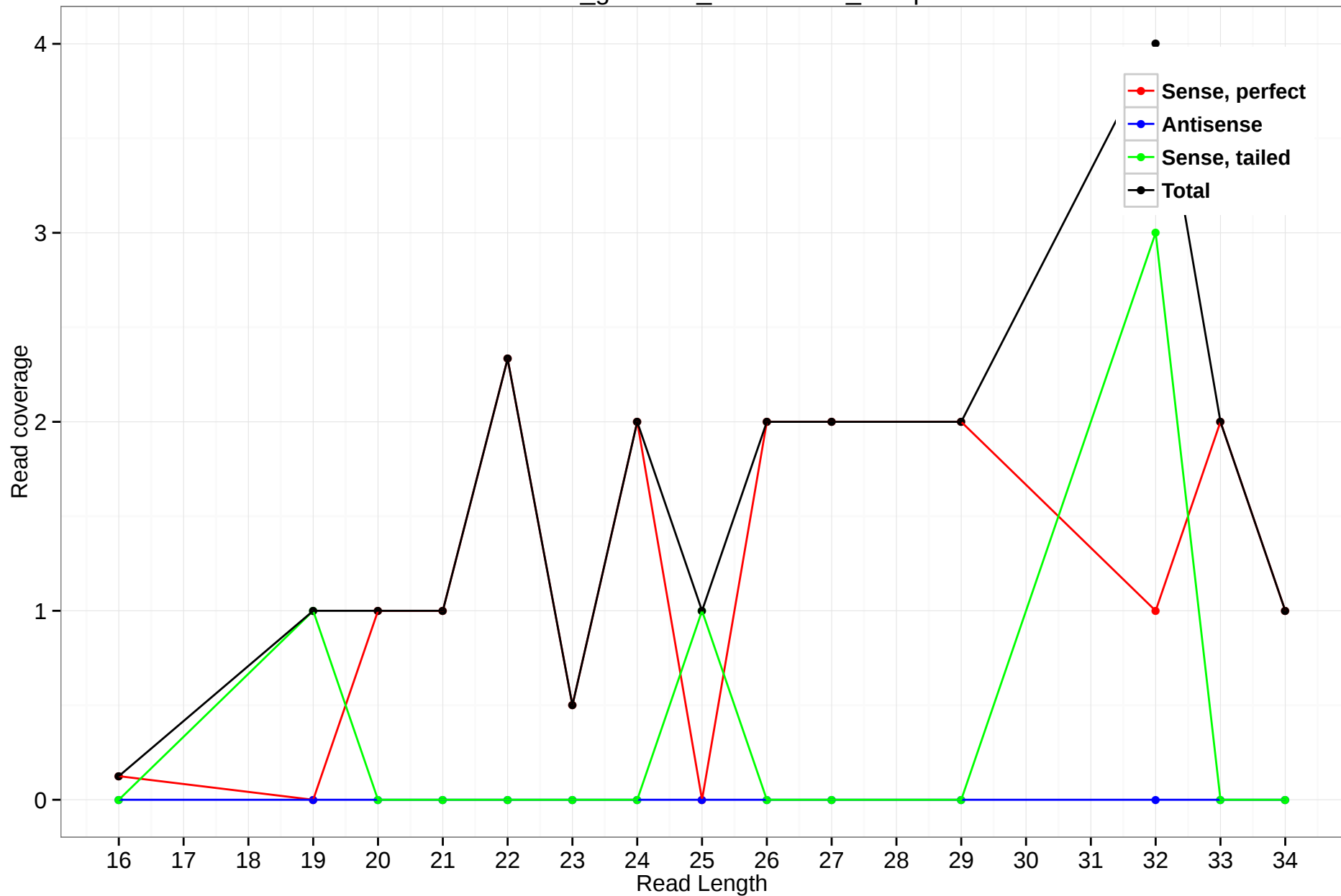
rheMac3_genscan_chr11.1941_17.3p
