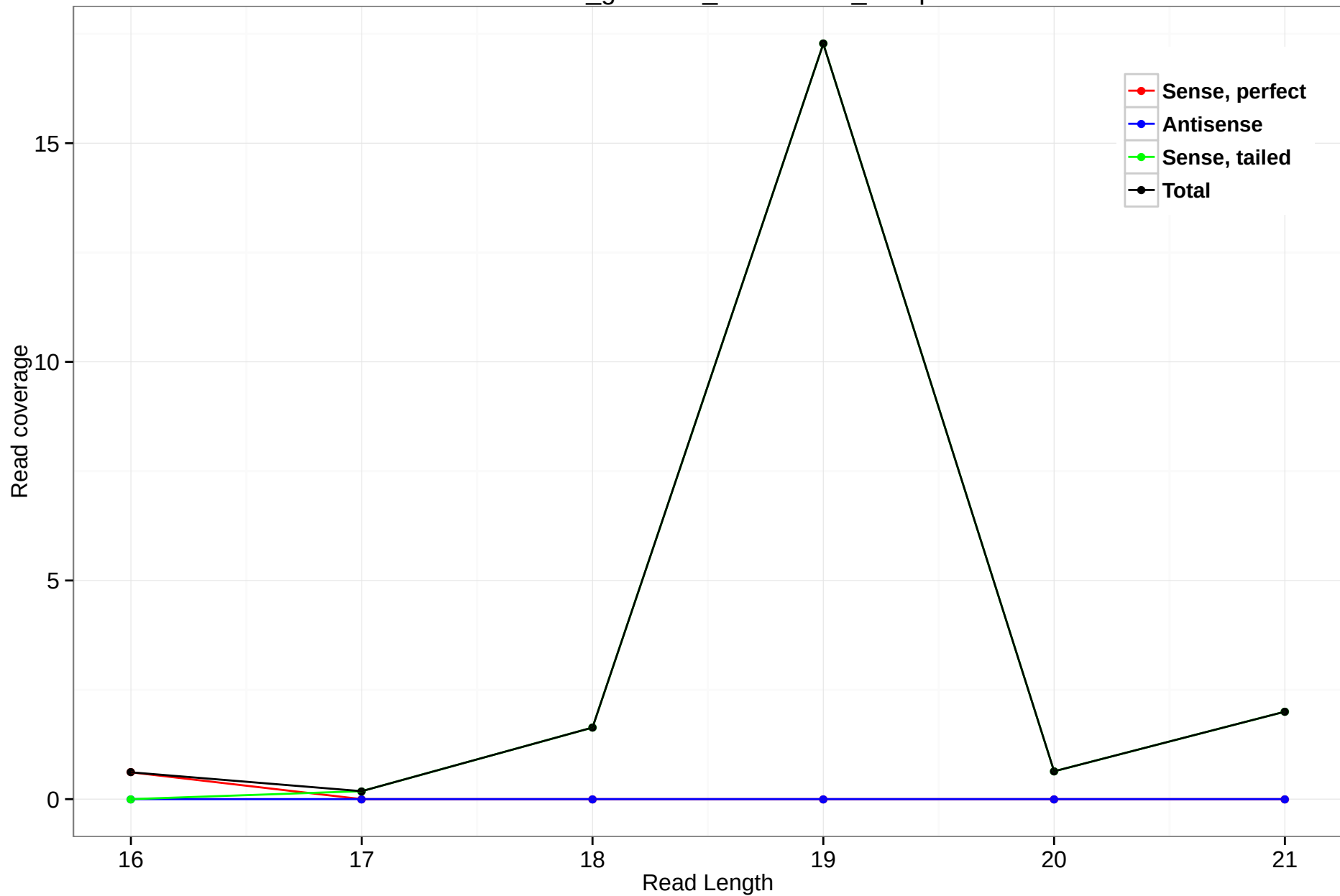
rheMac3_genscan_chr11.1939_17.5p
