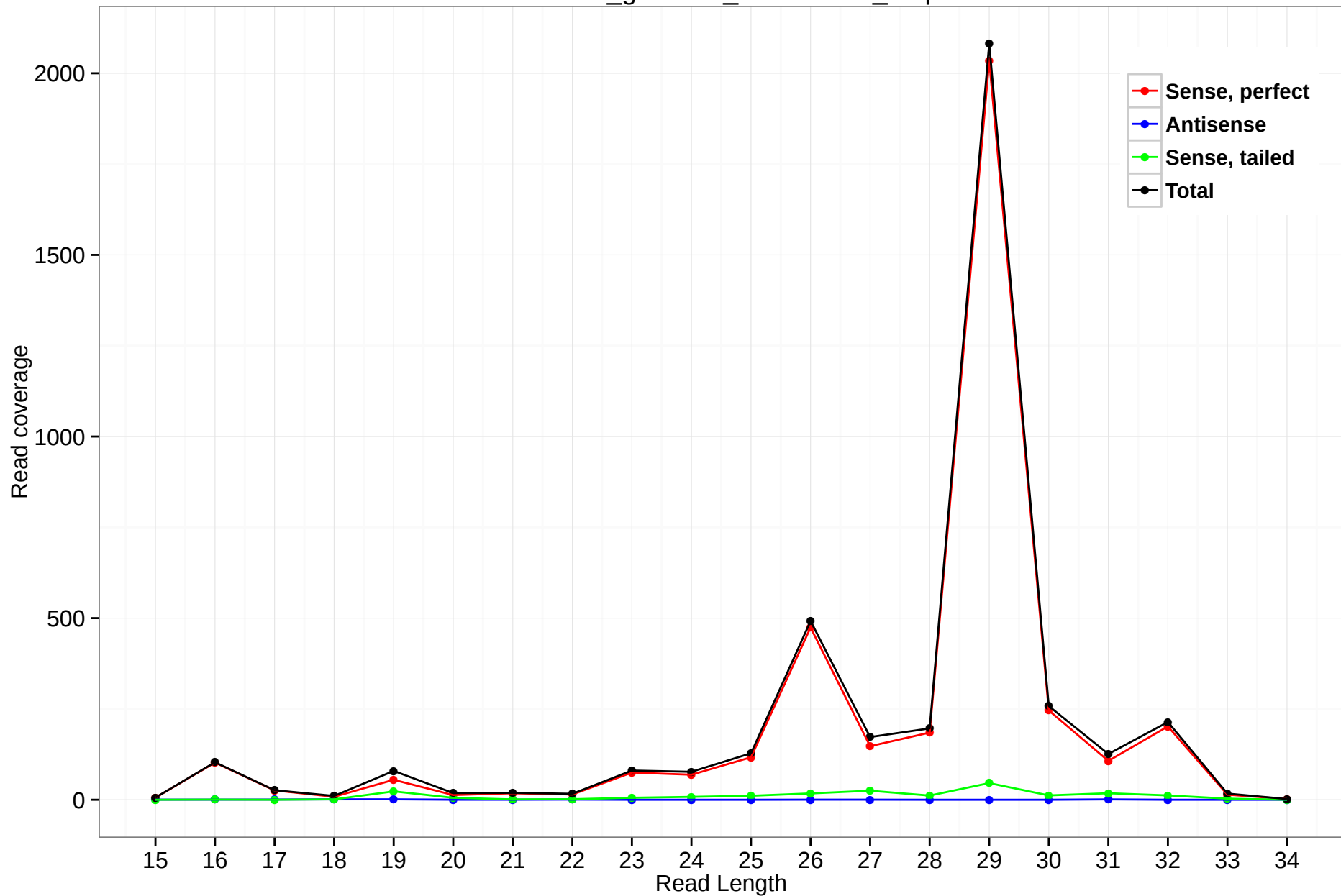
rheMac3_genscan_chr11.1877_9.5p
