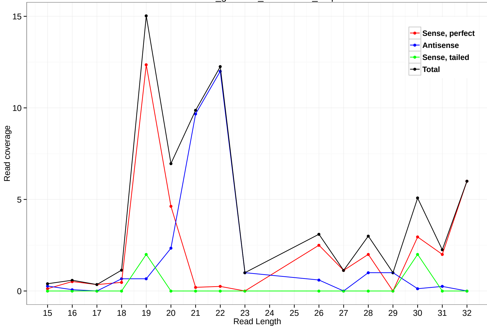
rheMac3_genscan_chr11.1877_6.5p
