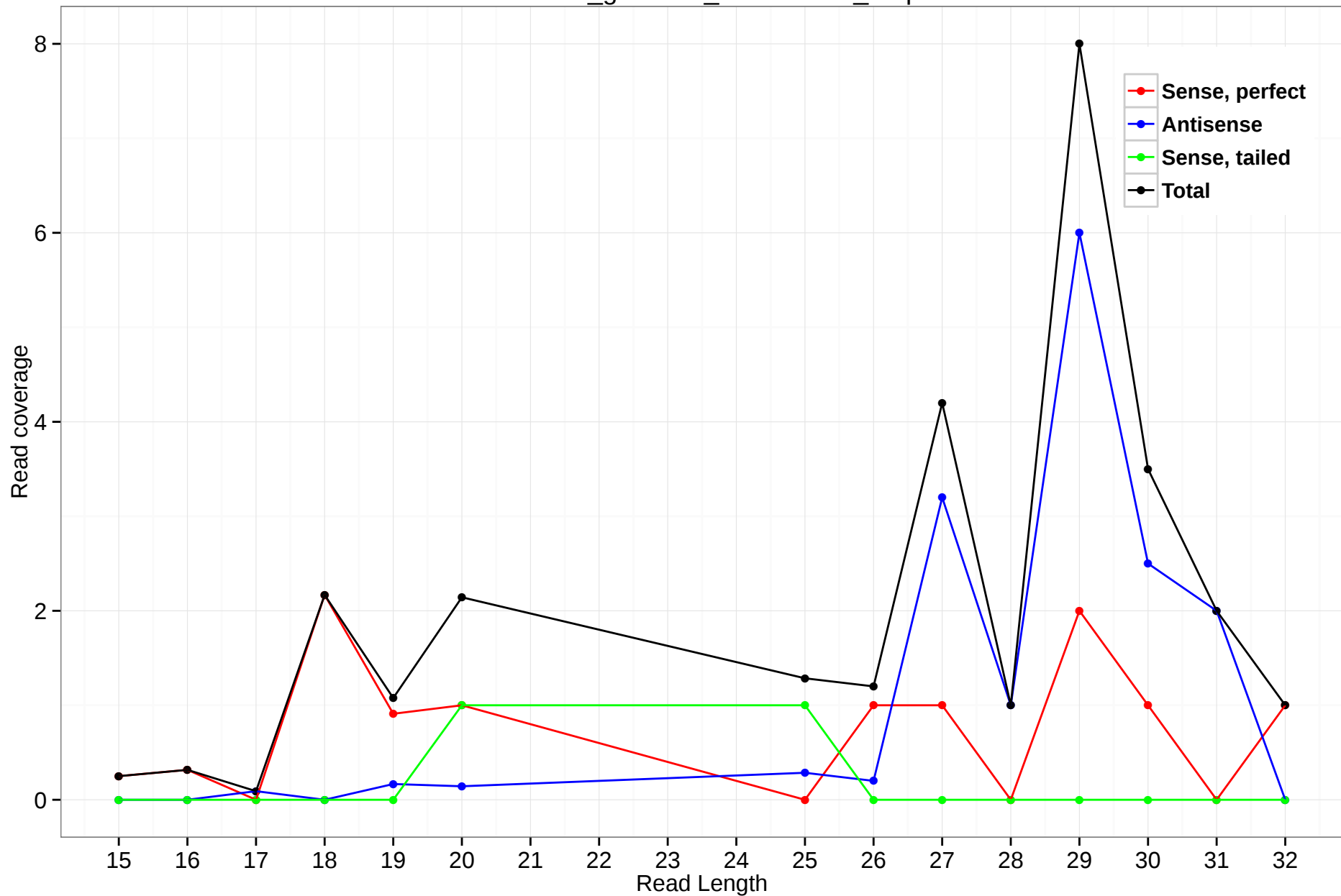
rheMac3_genscan_chr11.1877_5.3p
