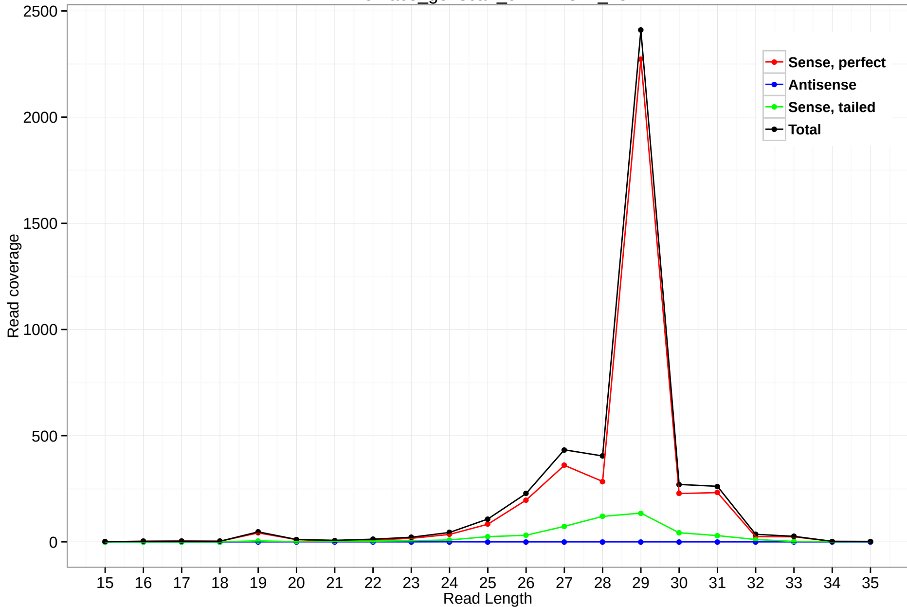
rheMac3_genscan_chr11.1877_15
