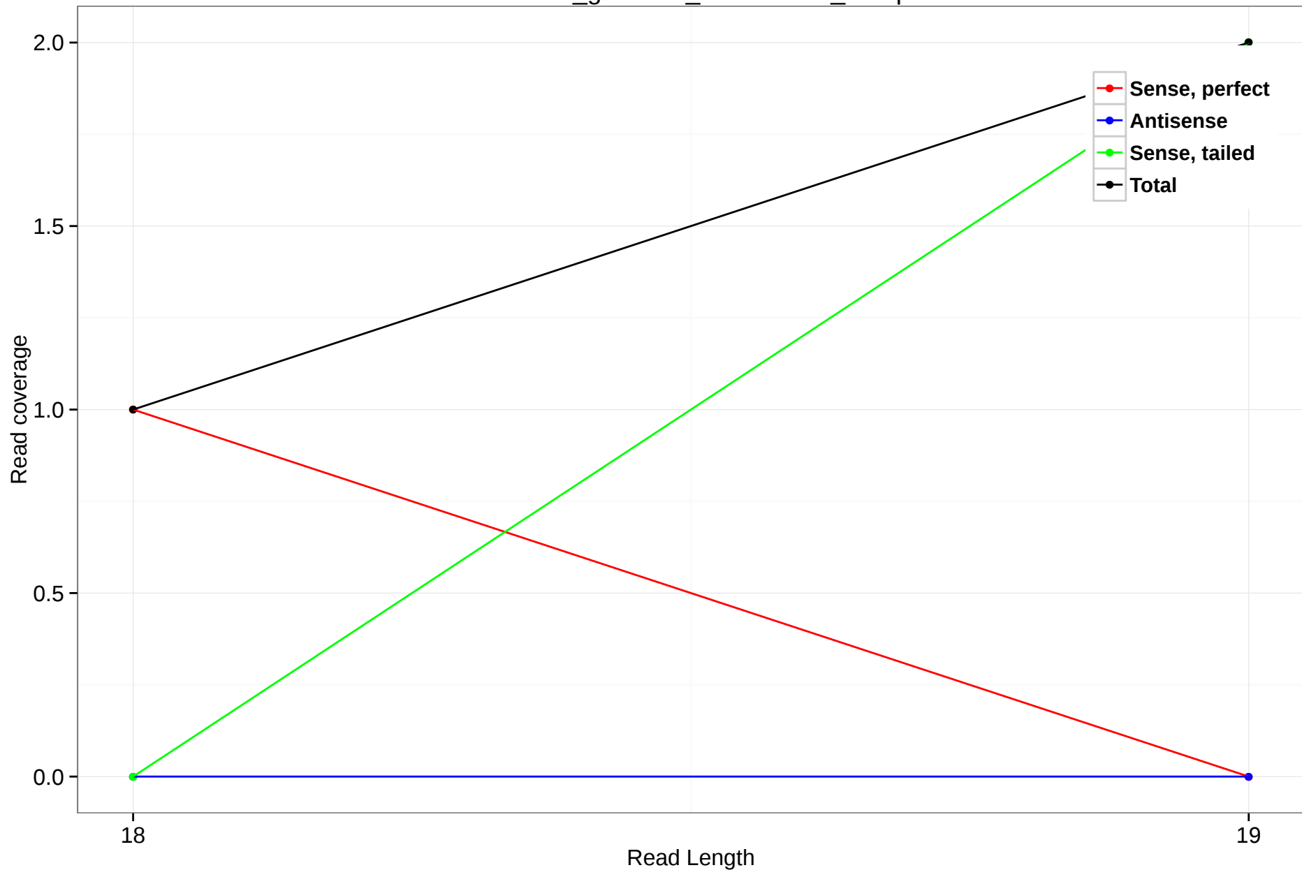
rheMac3_genscan_chr11.1859_23.3p
