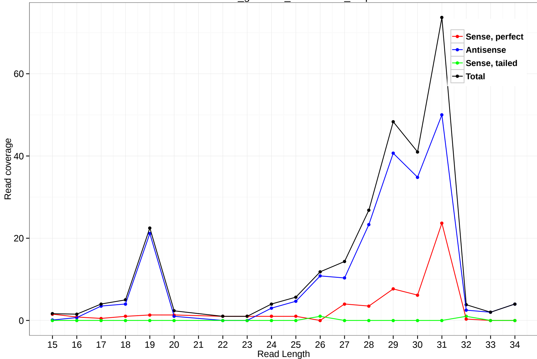
rheMac3_genscan_chr11.1855_0.3p
