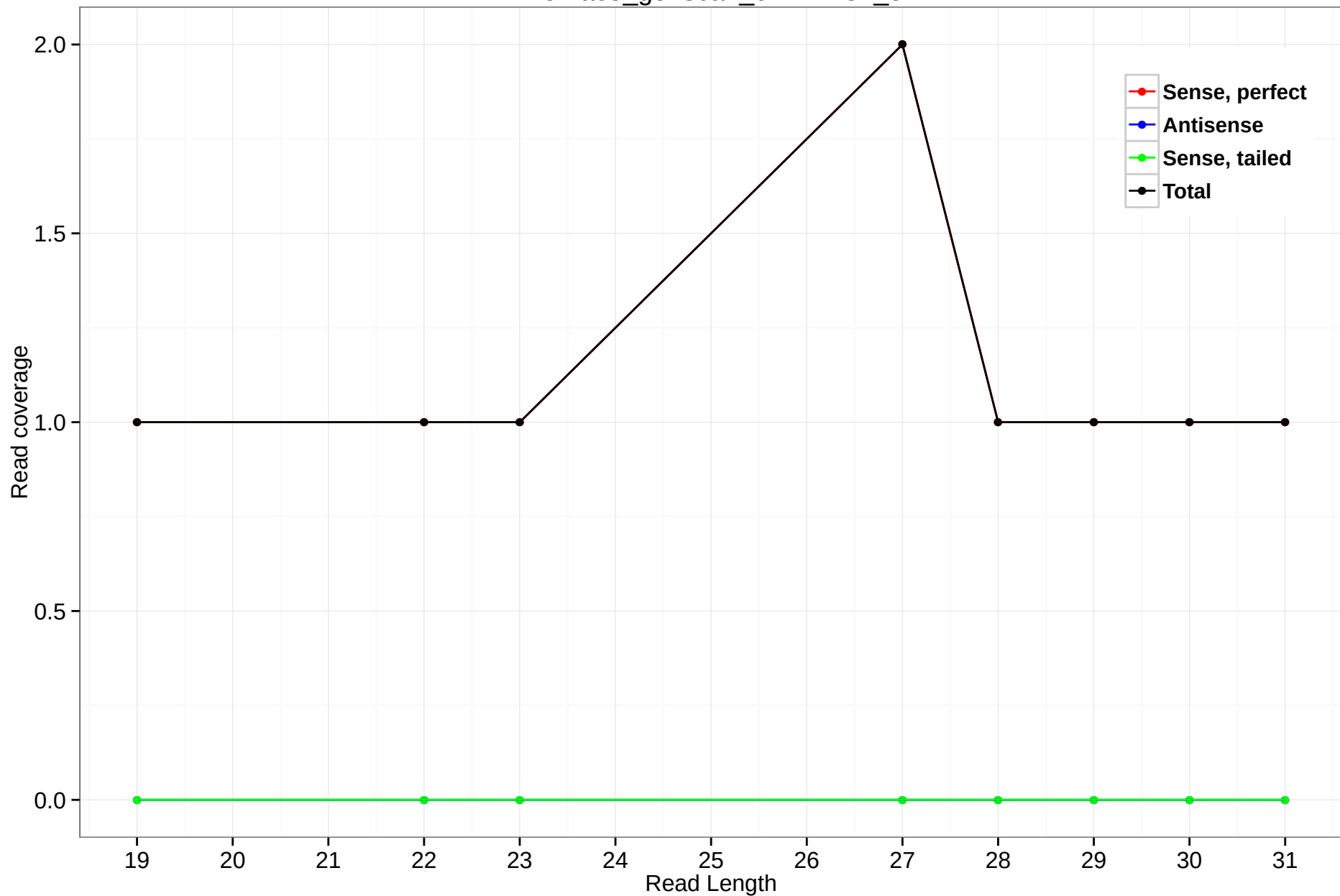
rheMac3_genscan_chr11.184_5
