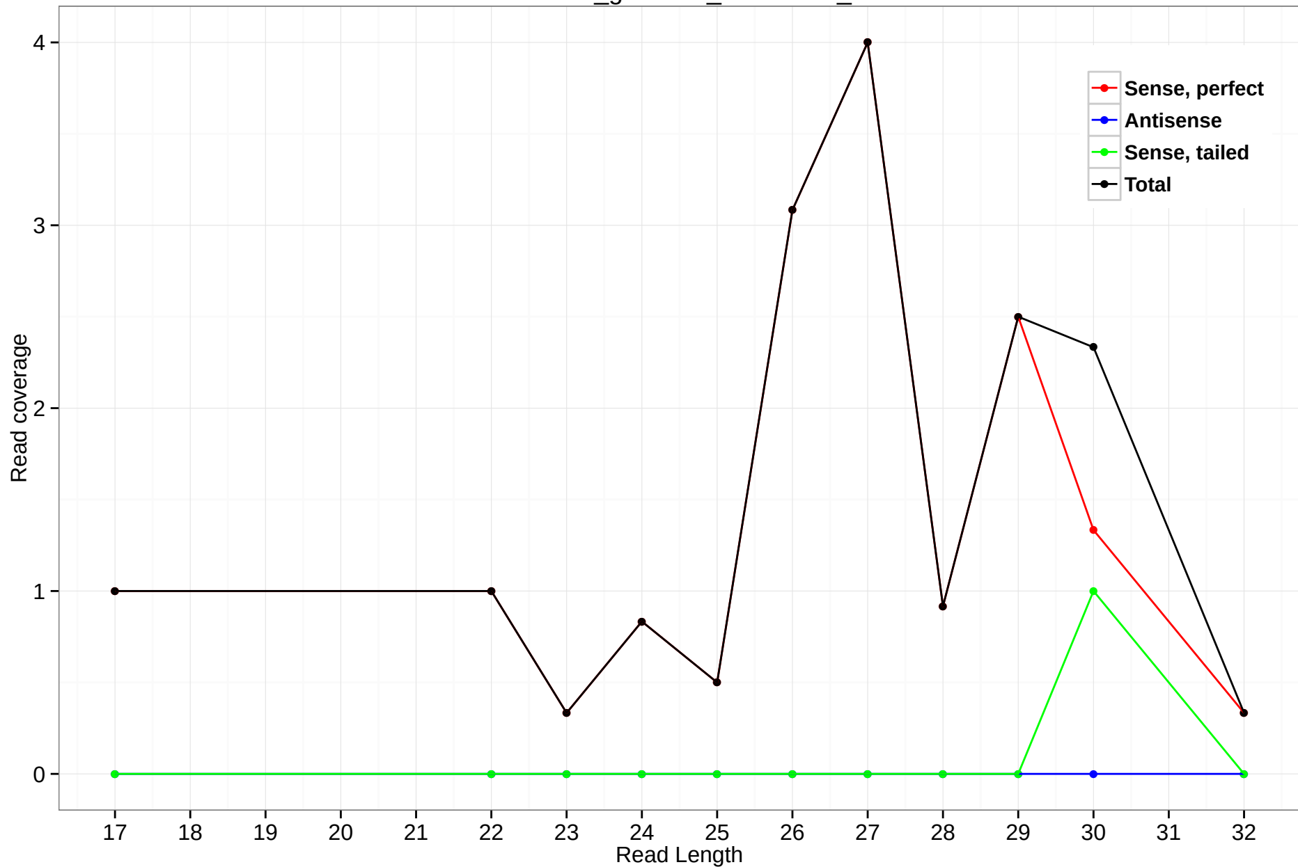
rheMac3_genscan_chr11.182_0
