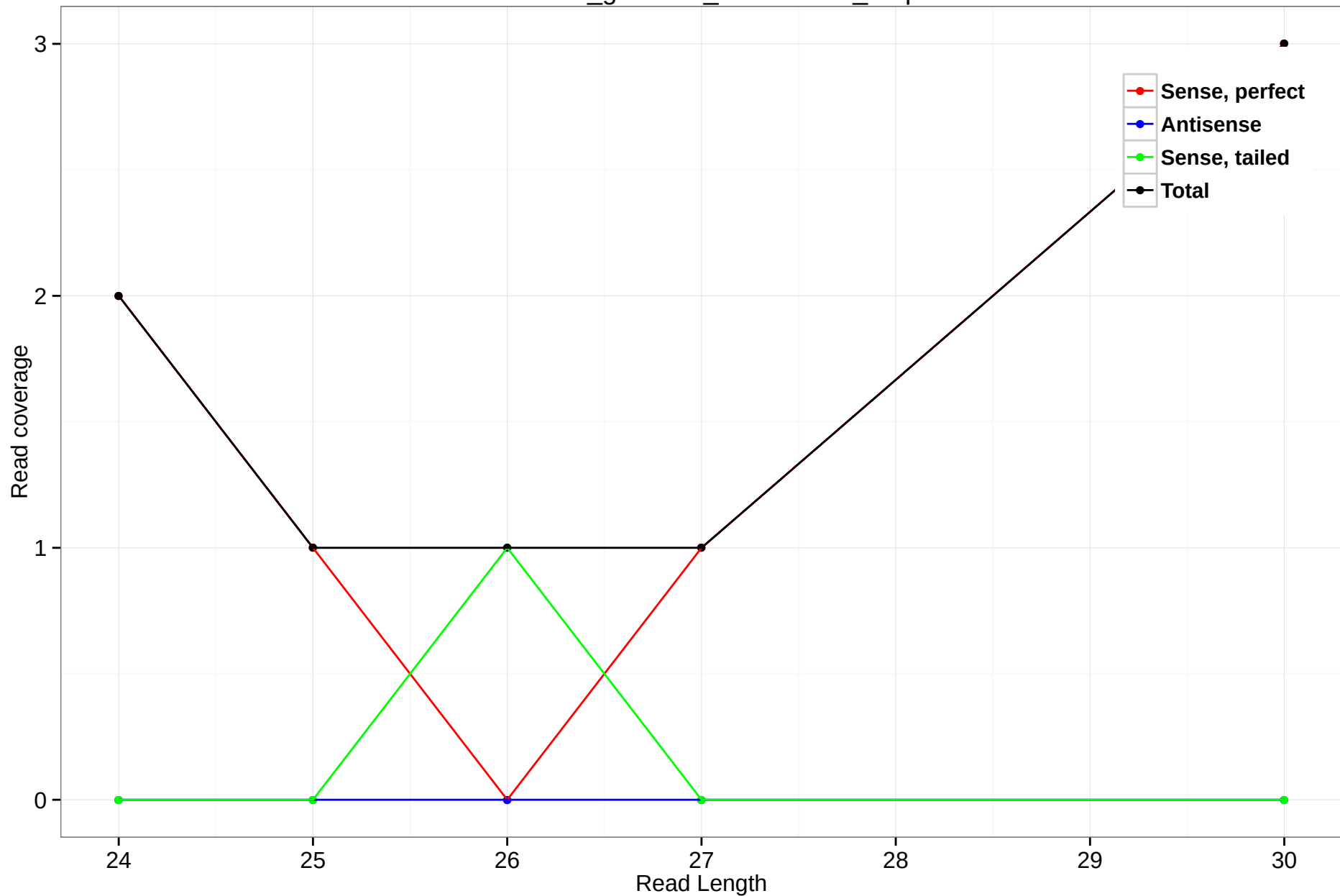
rheMac3_genscan_chr11.1774_4.3p
