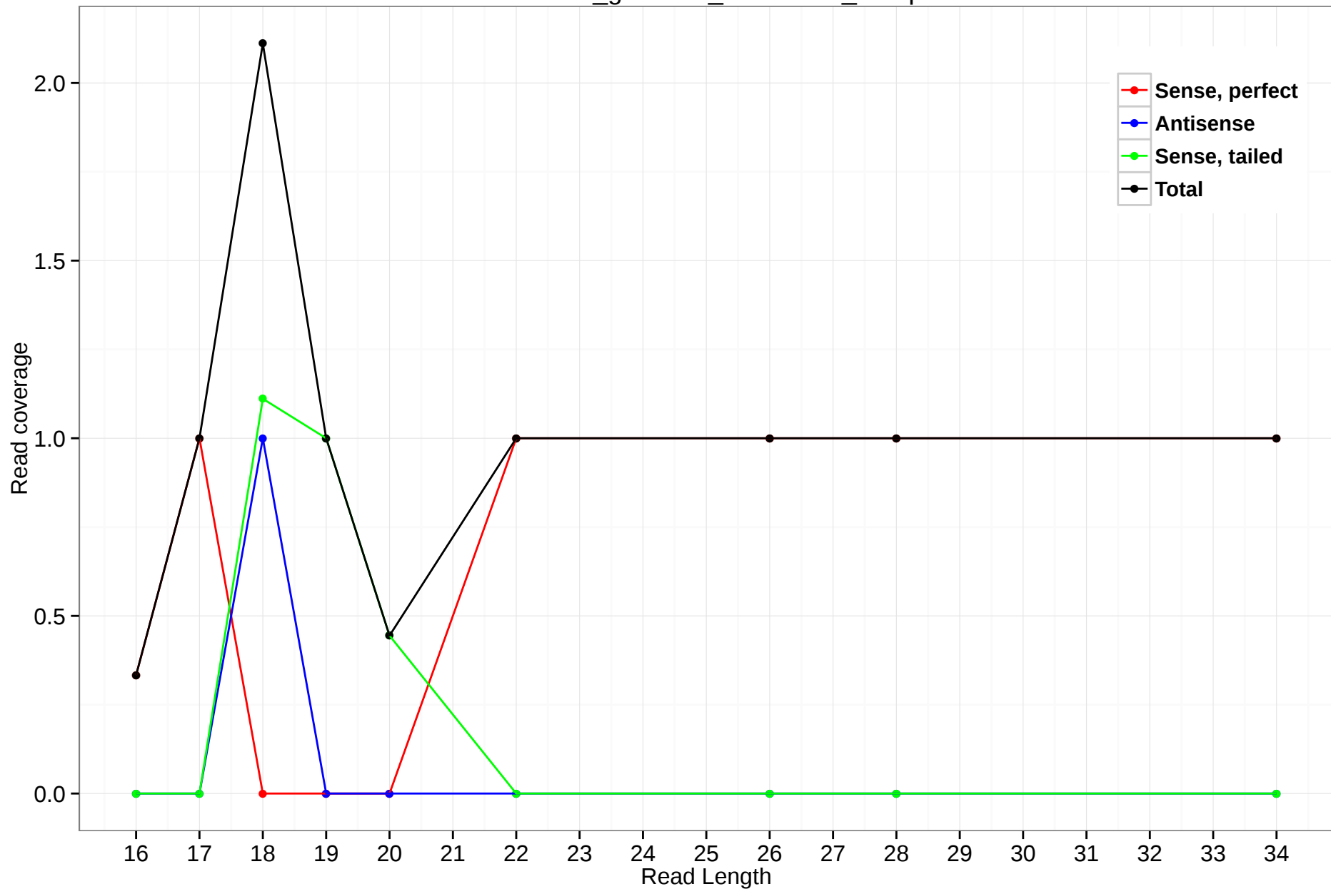
rheMac3_genscan_chr11.171_15.3p
