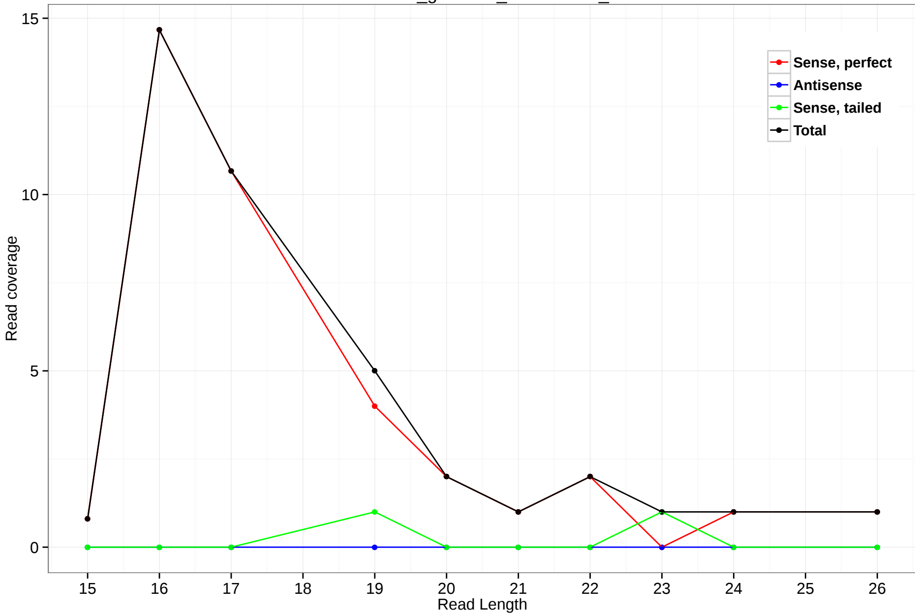
rheMac3_genscan_chr11.1691_5
