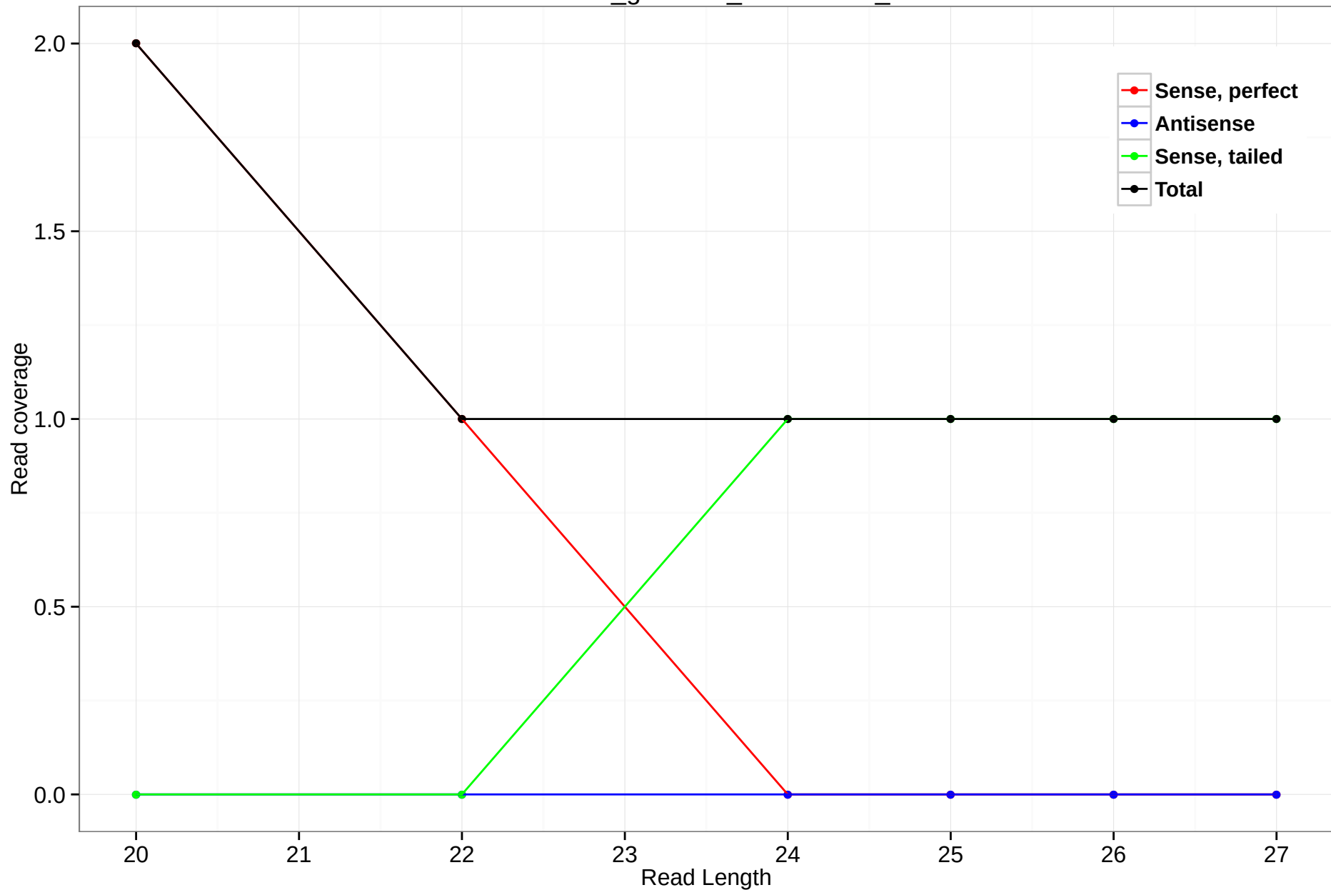
rheMac3_genscan_chr11.1649_9
