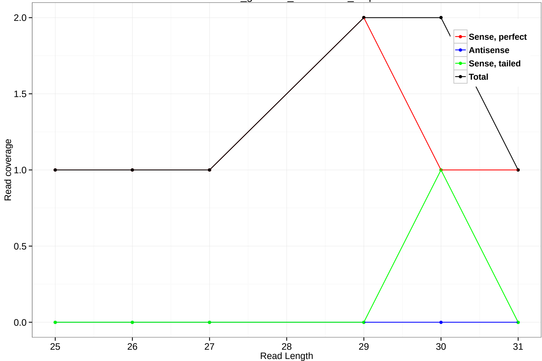
rheMac3_genscan_chr11.1647_2.3p
