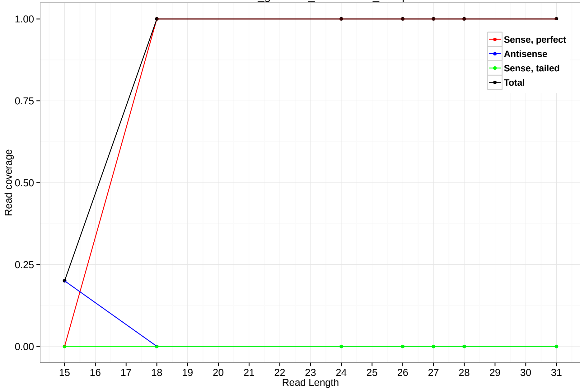
rheMac3_genscan_chr11.1647_19.5p
