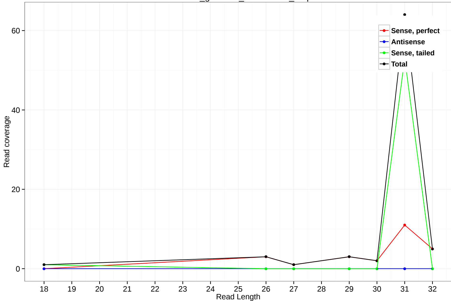
rheMac3_genscan_chr11.1646_8.5p
