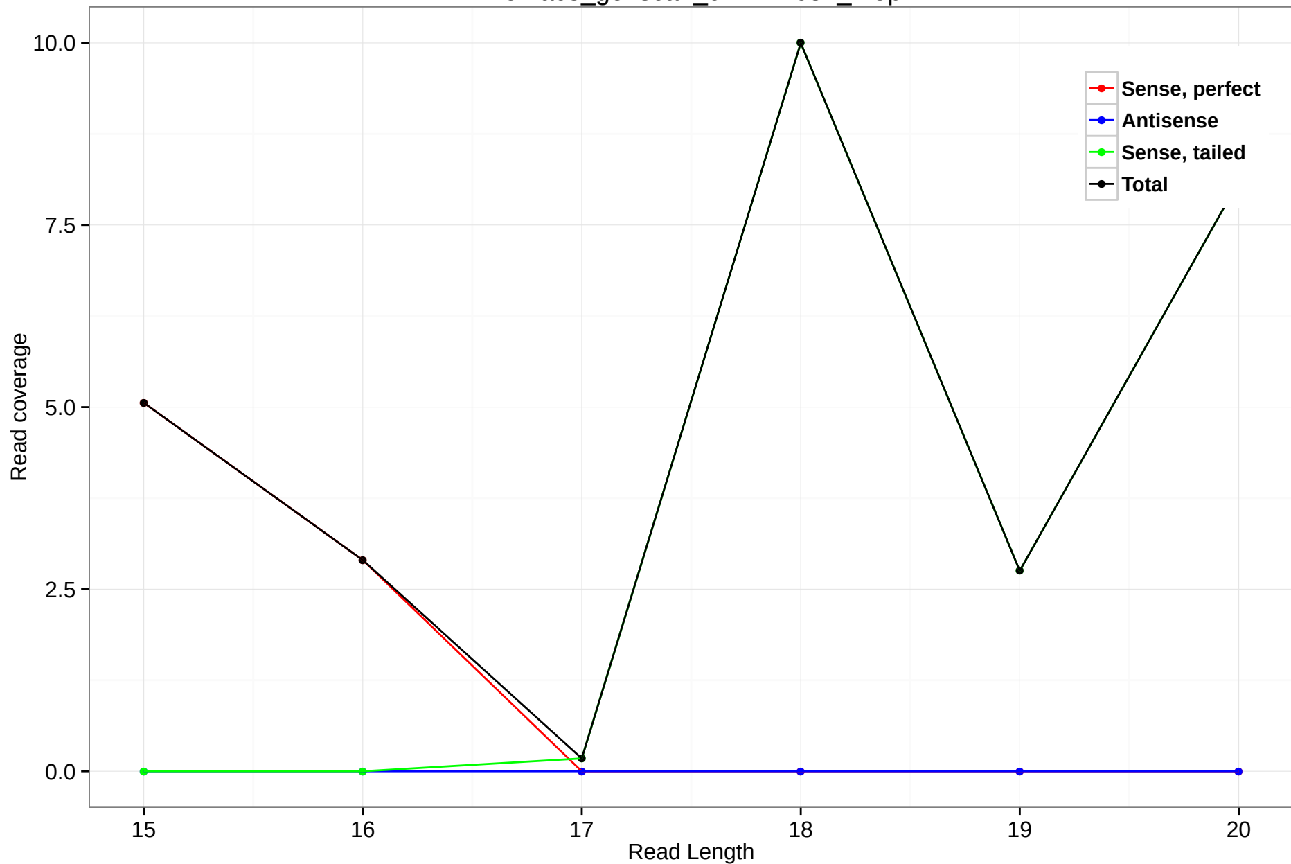
rheMac3_genscan_chr11.1634_1.5p
