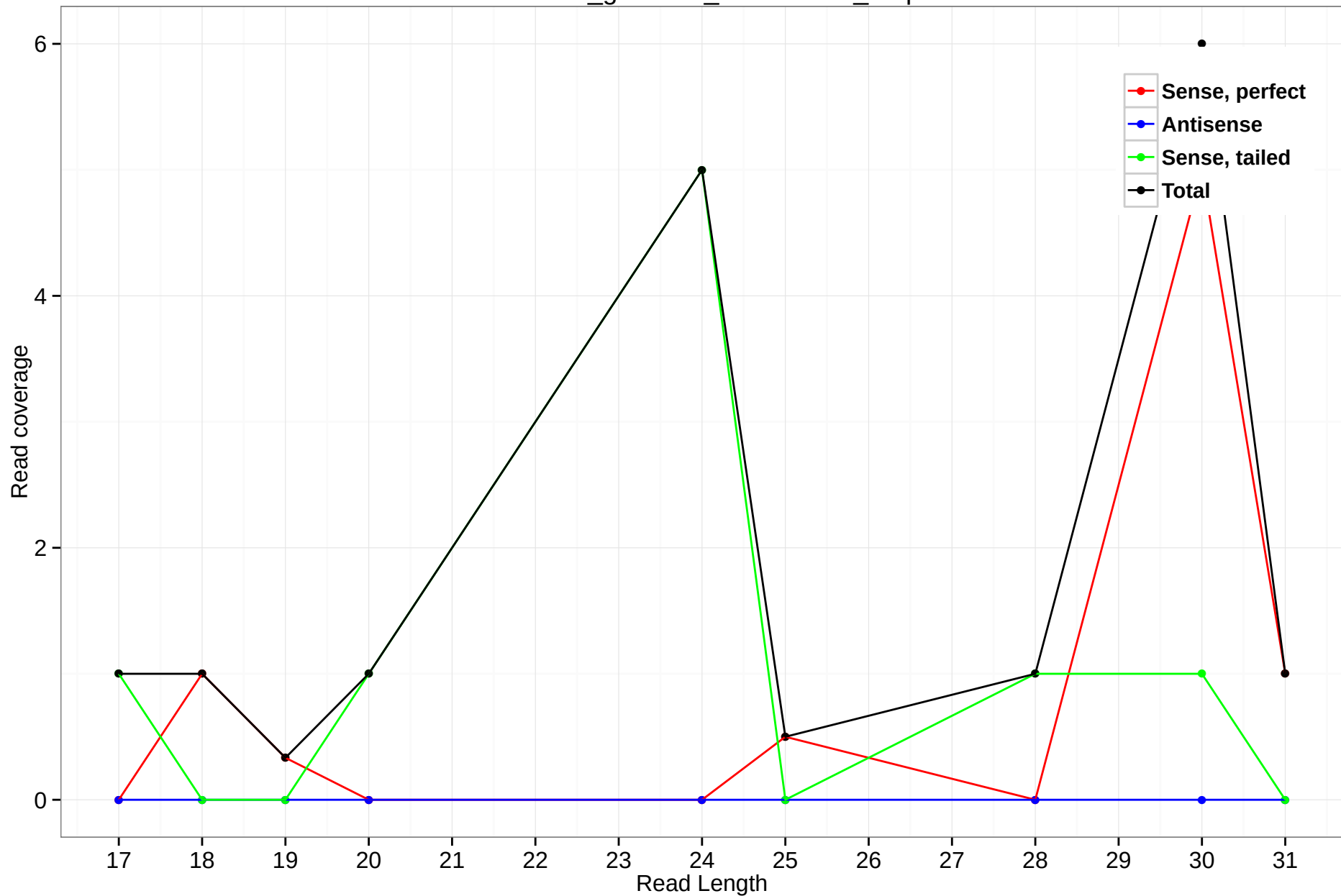
rheMac3_genscan_chr11.1600_0.3p
