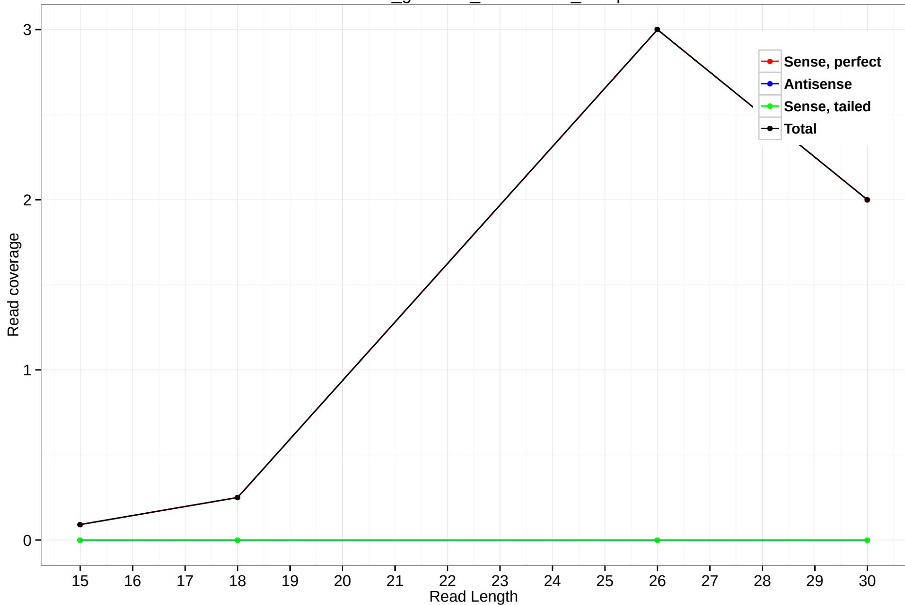
rheMac3_genscan_chr11.1571_11.5p
