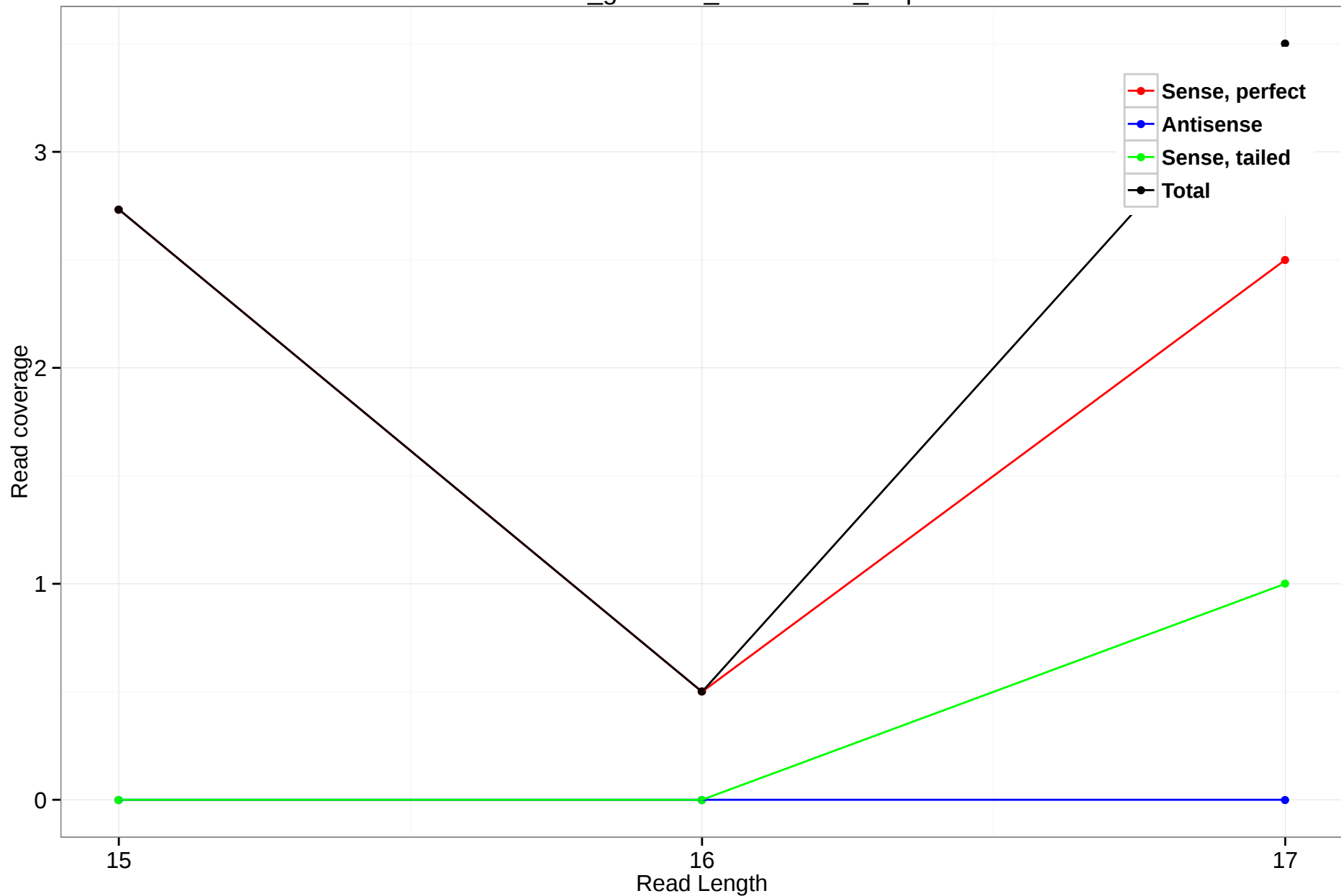
rheMac3_genscan_chr11.1562_3.5p
