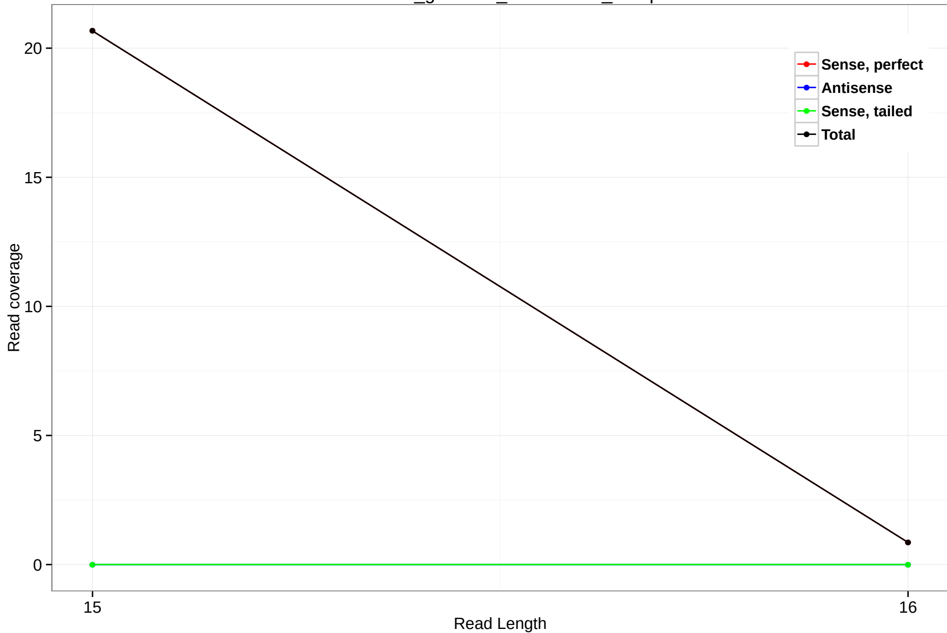
rheMac3_genscan_chr11.1507_27.3p
