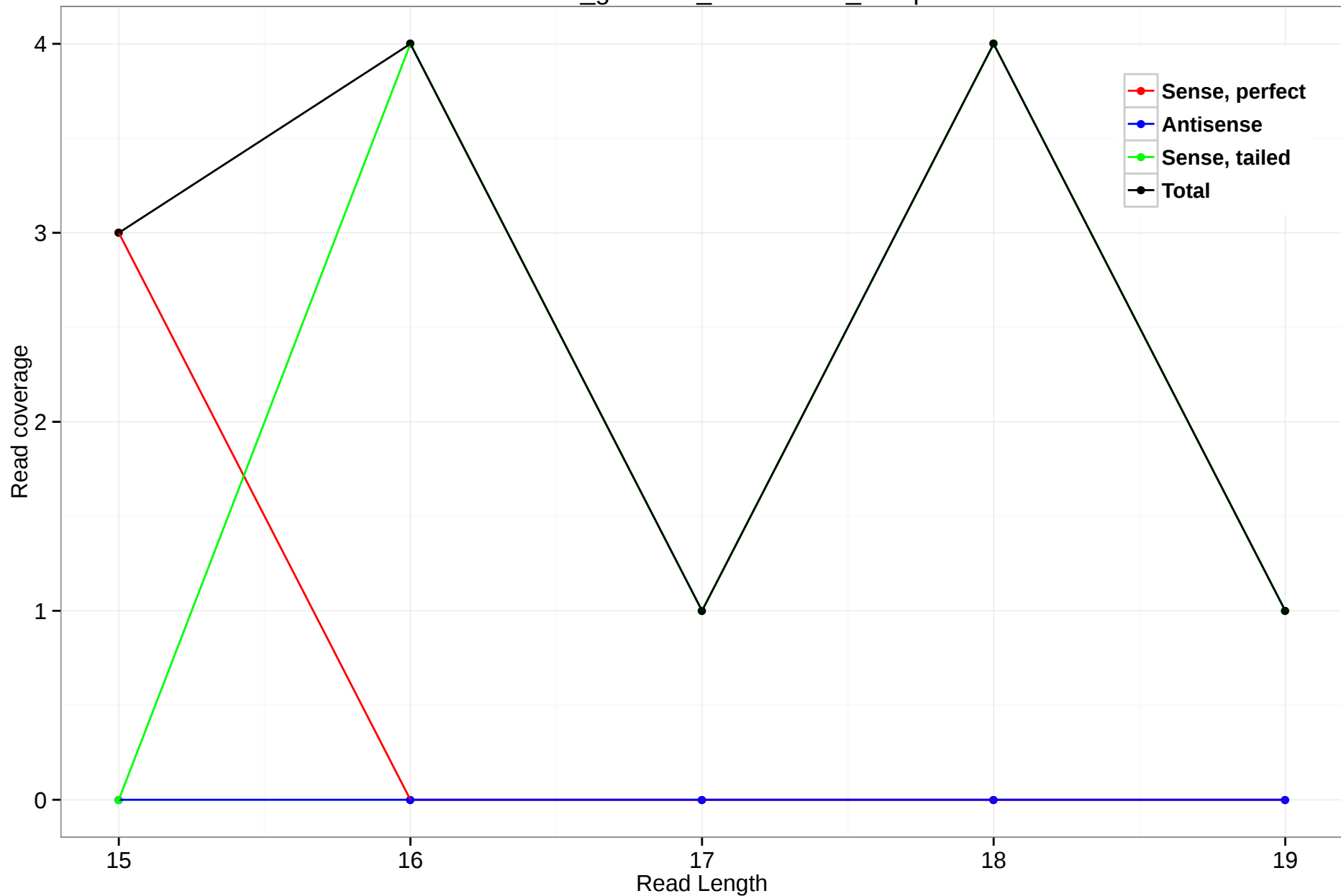
rheMac3_genscan_chr11.1507_24.3p
