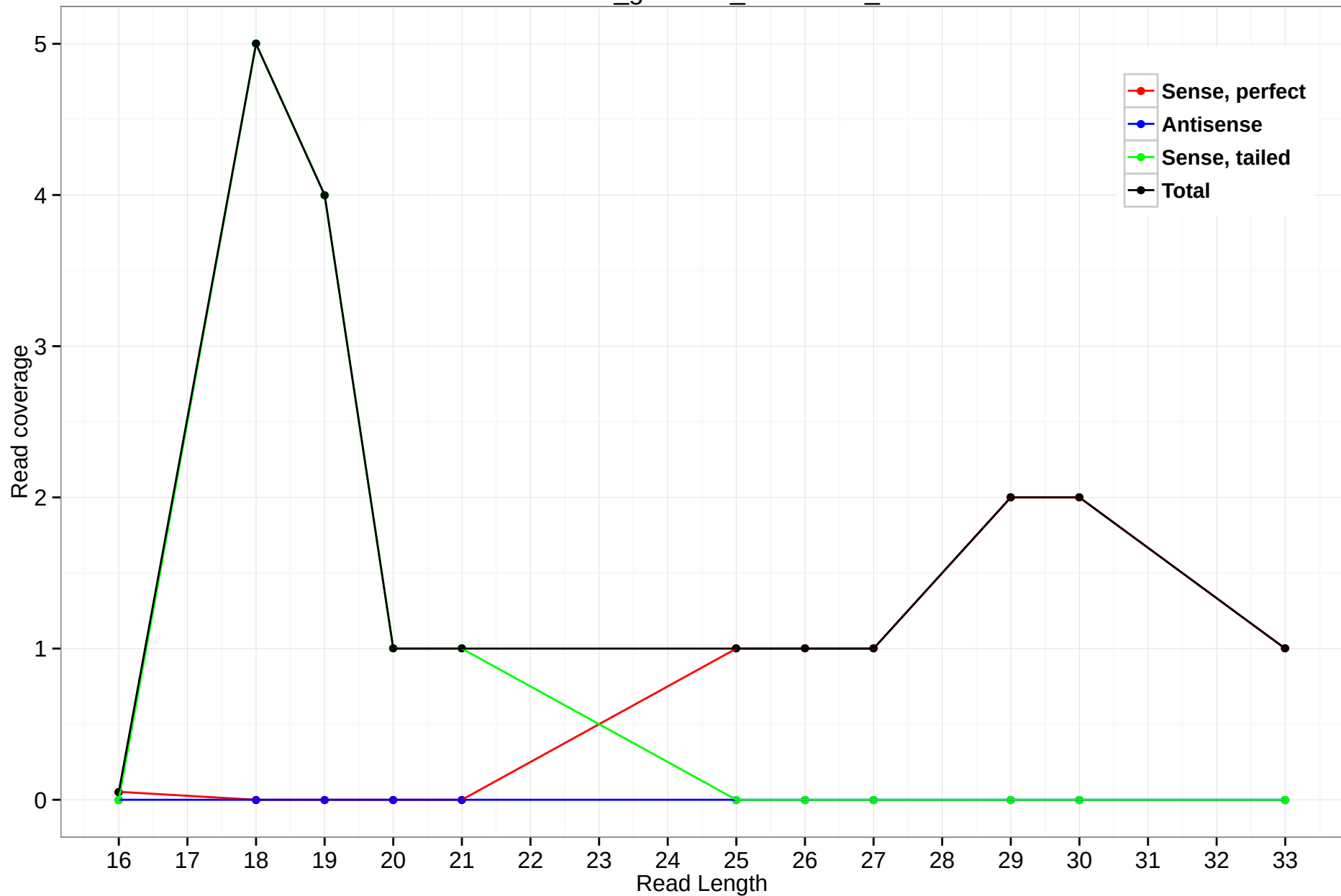
rheMac3_genscan_chr11.143_2
