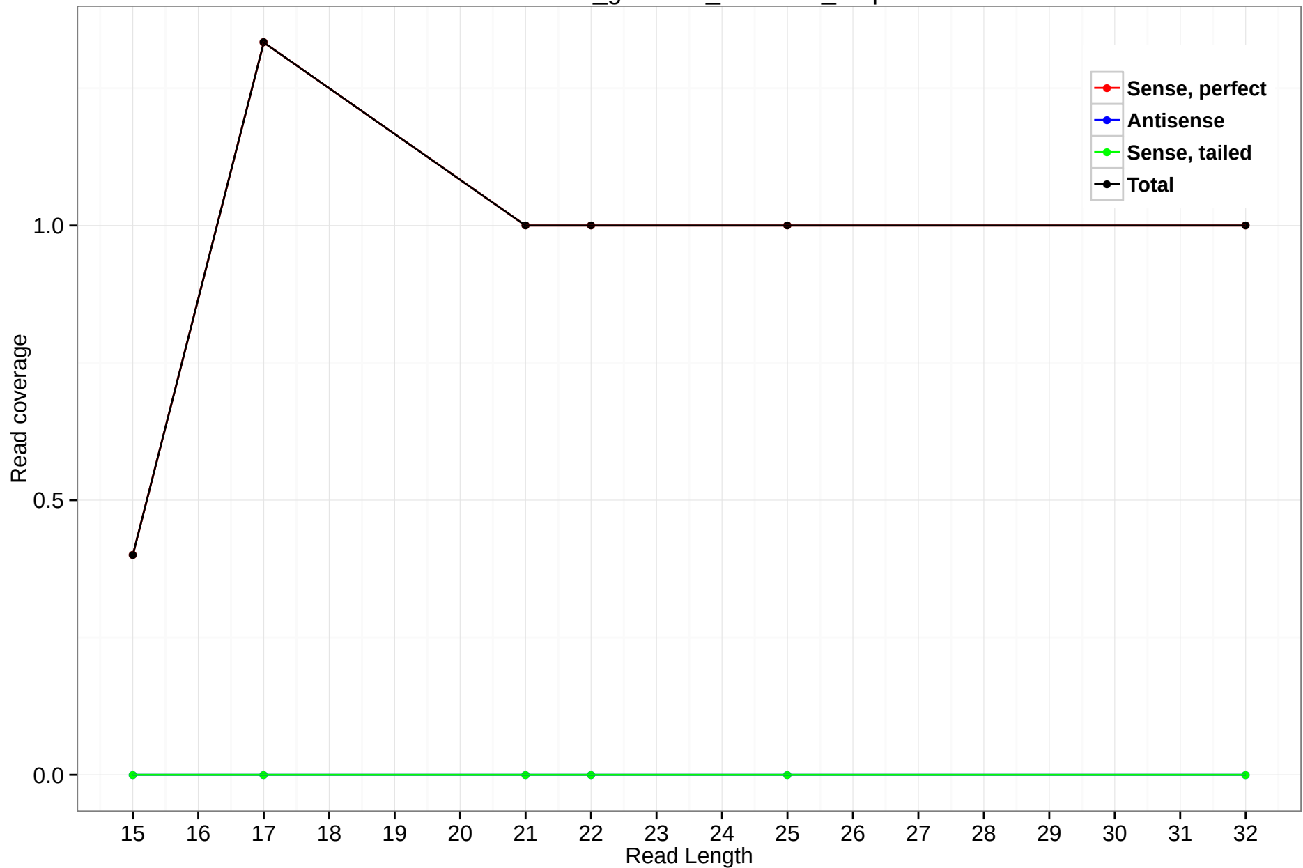
rheMac3_genscan_chr11.13_1.5p
