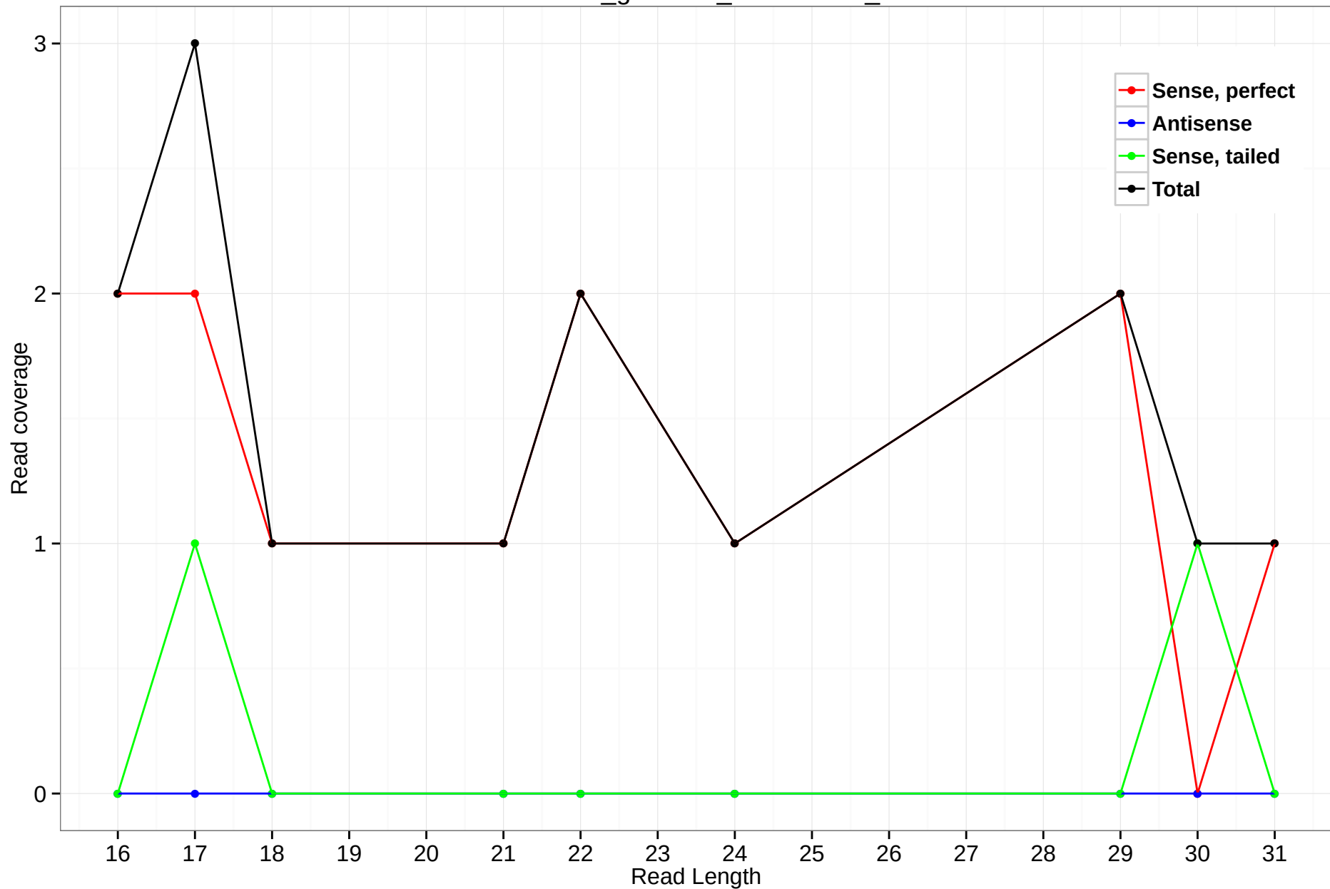
rheMac3_genscan_chr11.1395_1
