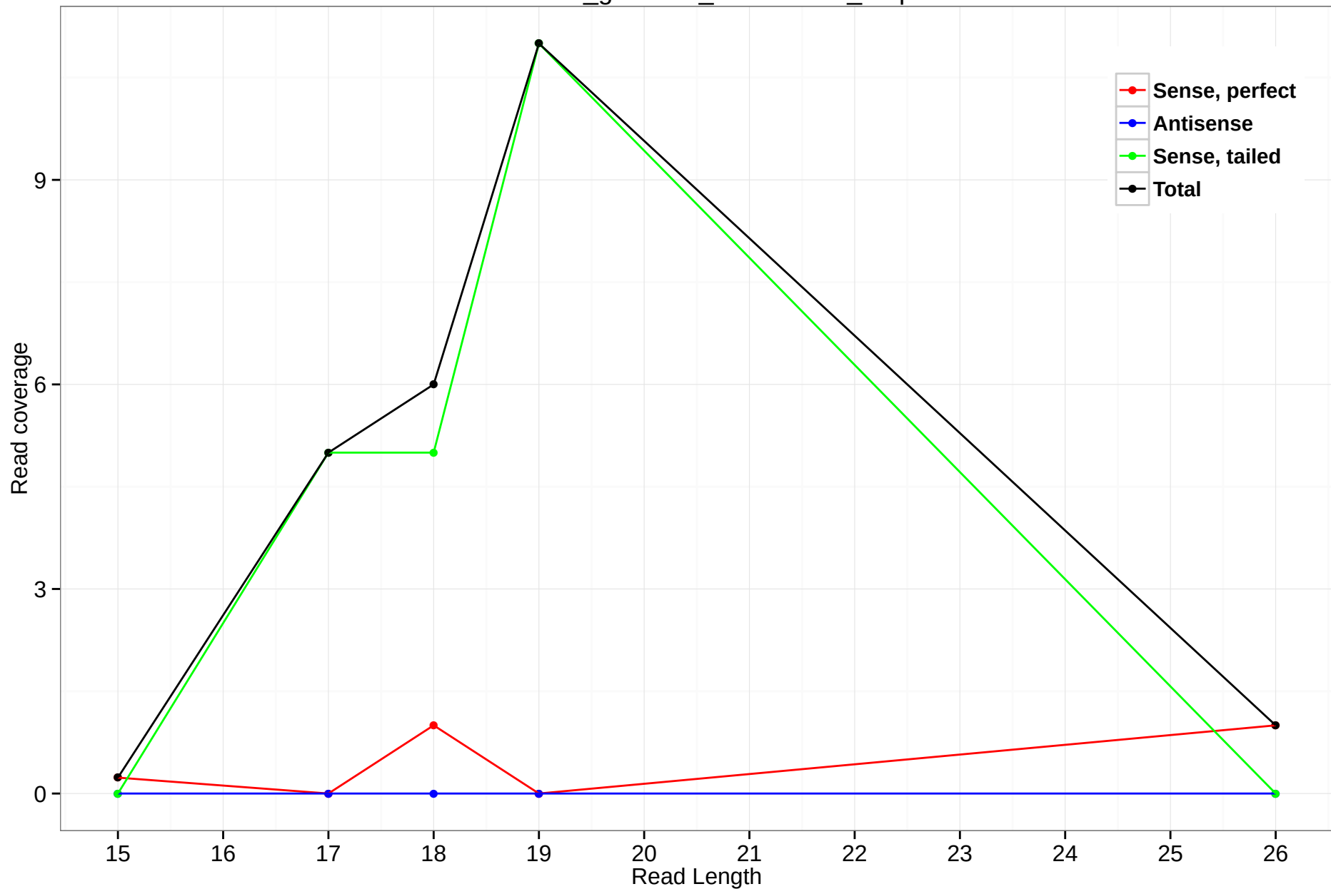
rheMac3_genscan_chr11.1386_8.3p
