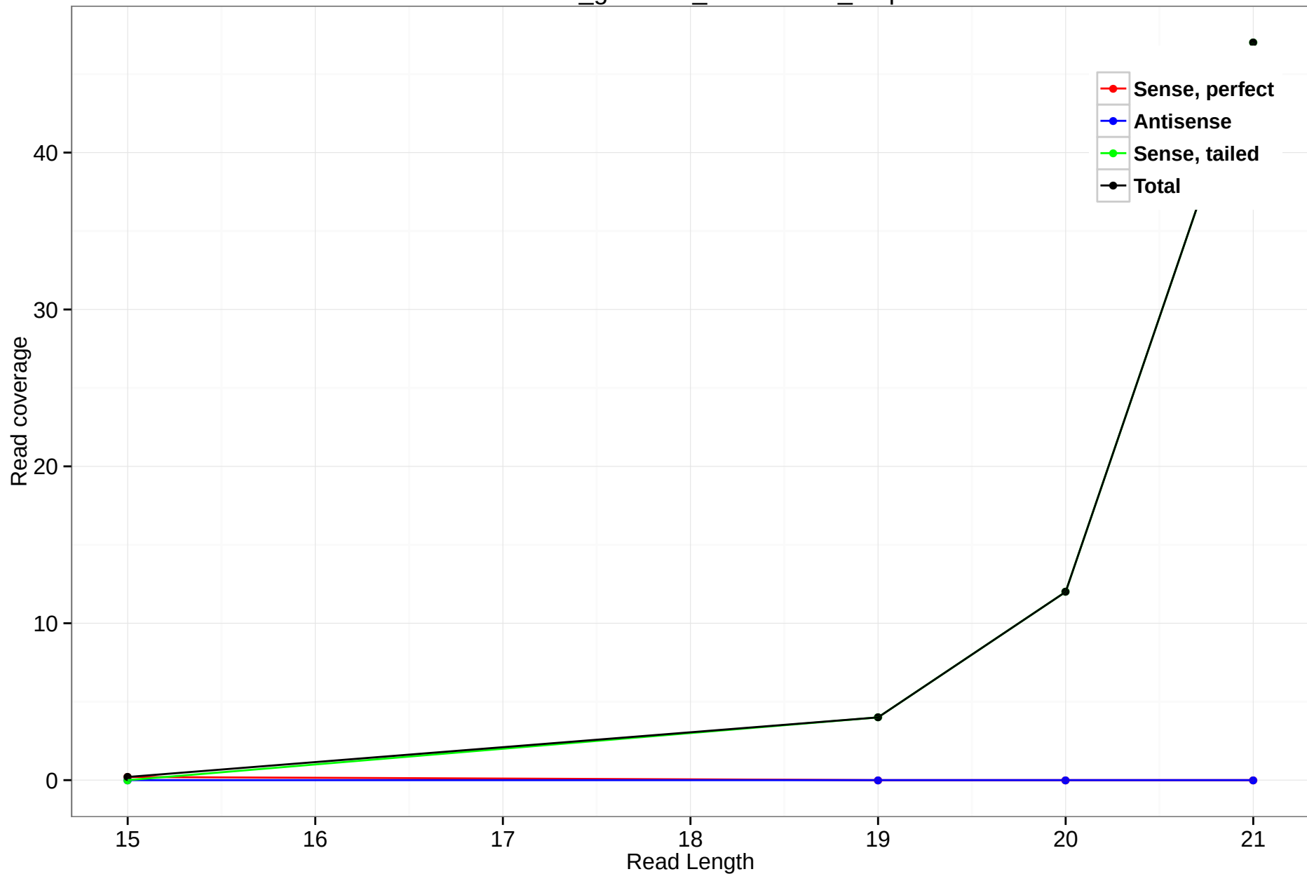
rheMac3_genscan_chr11.1250_5.5p
