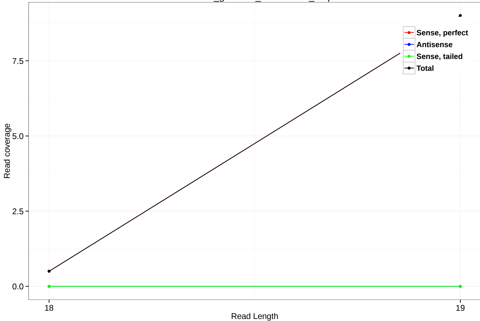
rheMac3_genscan_chr11.1193_0.3p
