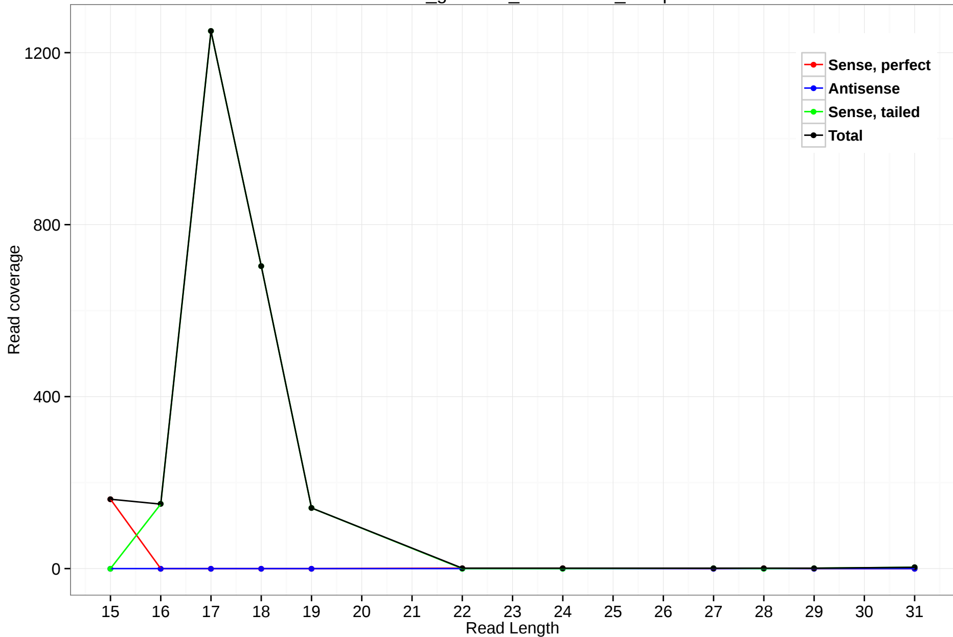
rheMac3_genscan_chr11.1146_13.5p
