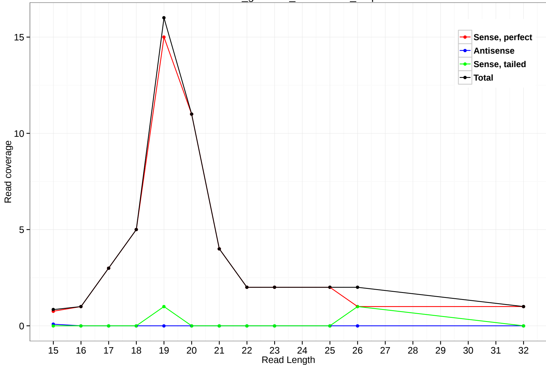
rheMac3_genscan_chr11.1144_2.5p
