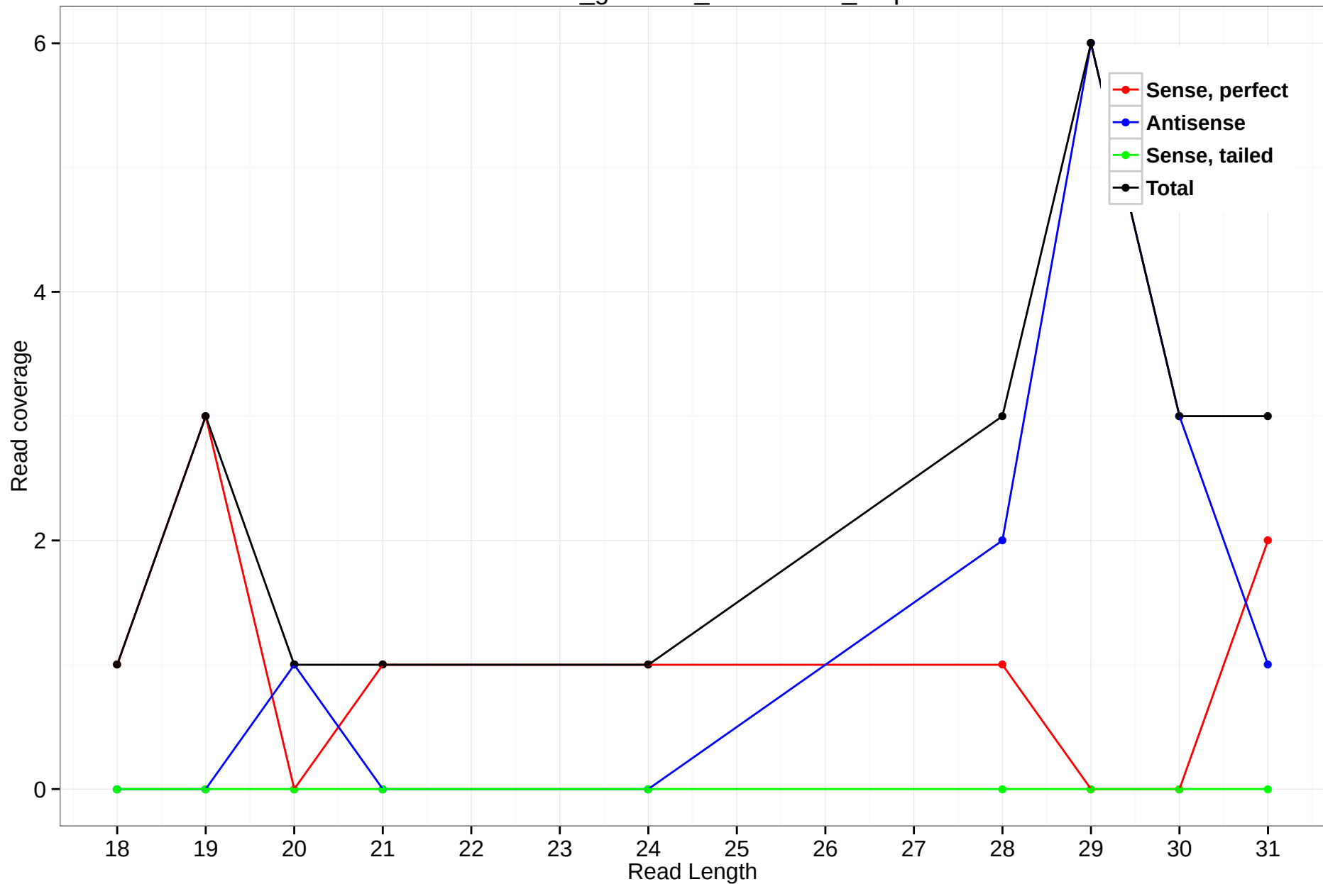
rheMac3_genscan_chr11.1144_0.5p
