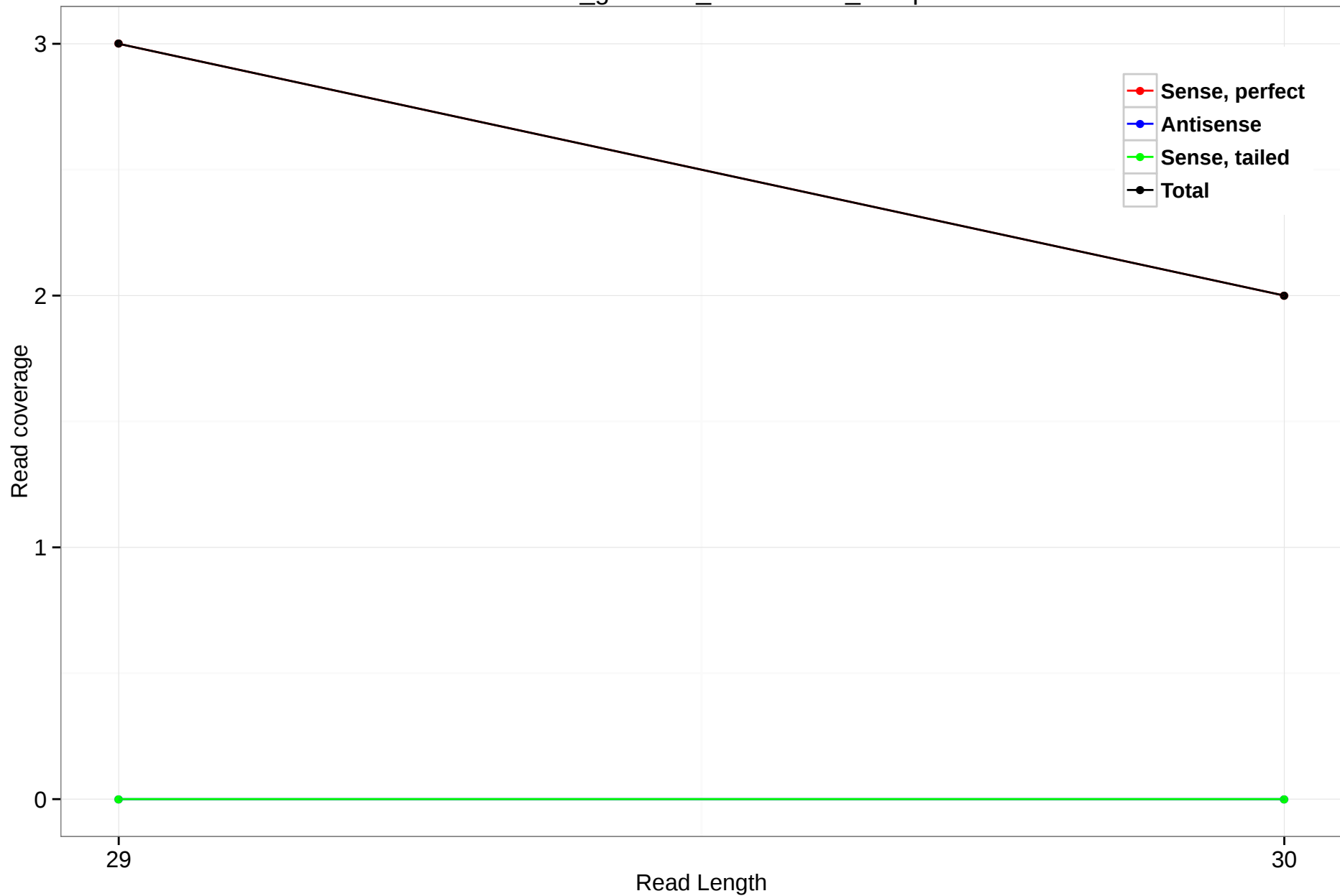
rheMac3_genscan_chr11.1099_34.5p
