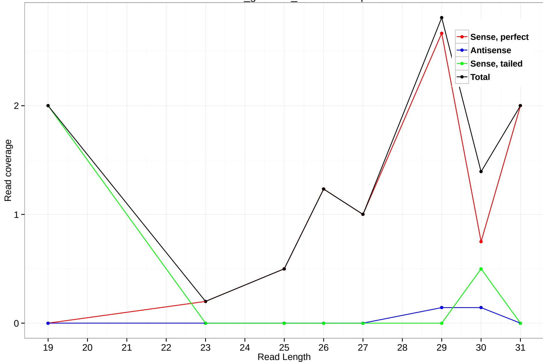
rheMac3_genscan_chr11.1033.3p
