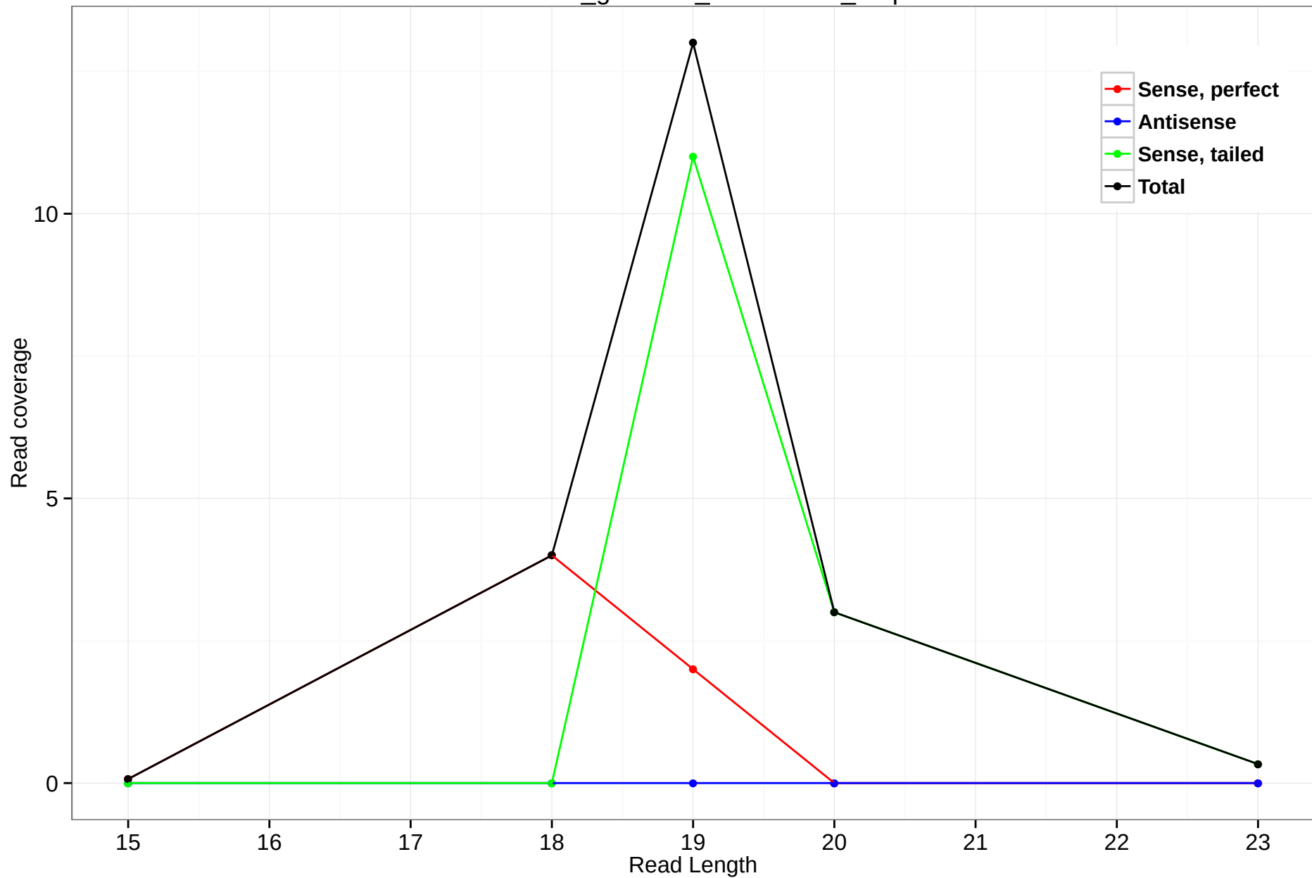
rheMac3_genscan_chr11.1020_0.5p
