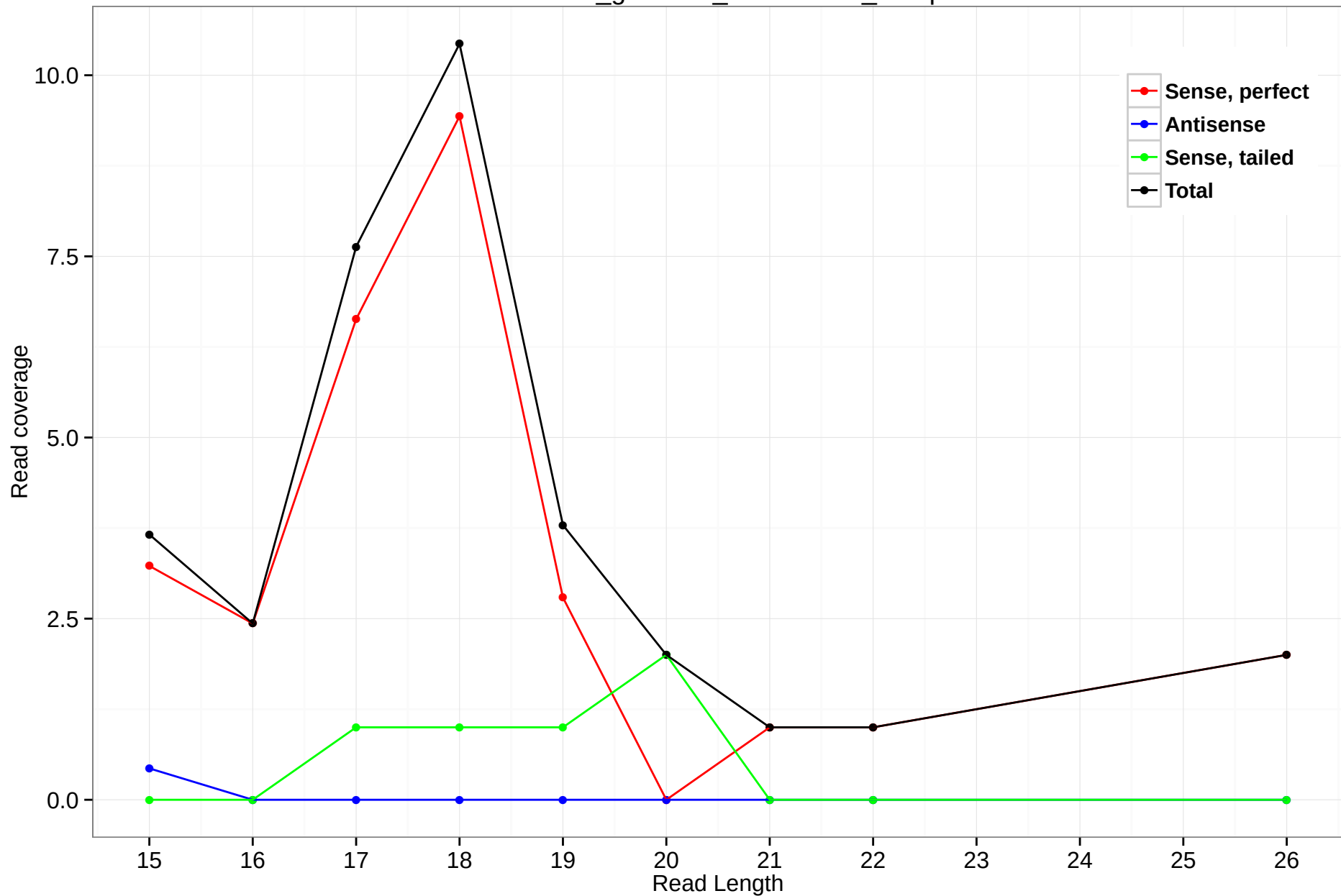
rheMac3_genscan_chr11.1016_30.3p
